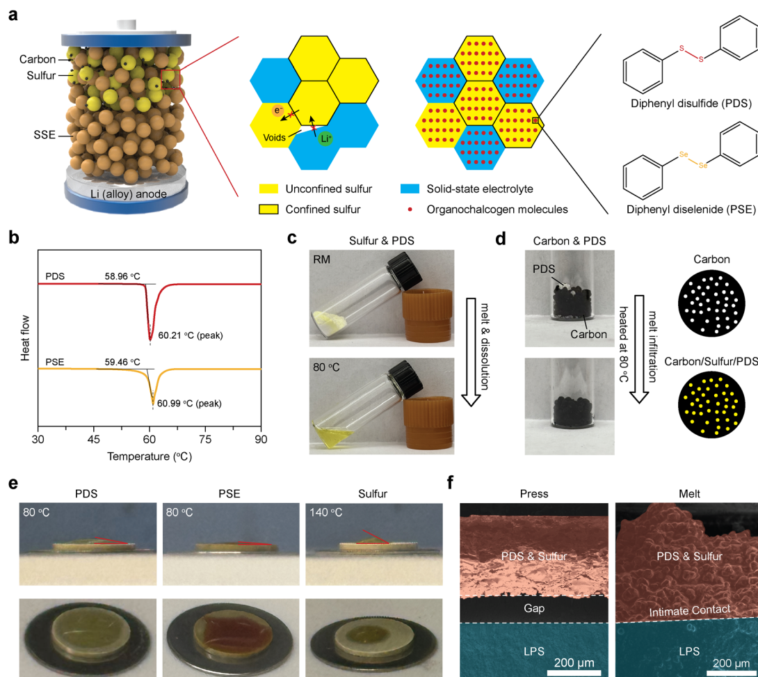
Fig. 1 Triphilic nature of organochalcogen compounds. (a) Schematic illustration of the mechanism of triphilic organochalcogen molecules (i.e., PDS and PSE) in promoting uniformity and facilitating favorable interfacial contact among cathode components. (b) DSC curves of PDS and PSE. (c) Photographs of the sulfur–PDS mixture before and after melting at 80 °C, demonstrating that sulfur can be dissolved into PDS melts. (d) Photographs of the carbon–PDS mixture before and after melt infiltration (heat treatment at 80 °C), along with a schematic illustration depicting the infiltration of PSE into the pores of porous carbon. (e) Contact angle measurements of PDS, PSE, and sulfur melts on the surface of the LPS pellet. The results show that PDS and PSE can wet the surface with smaller contact angles at 80 °C than molten sulfur at 140 °C. (f) SEM images of the PDS–sulfur mixture and LPS pellets before (left) and after heat treatment at 80 °C (right). The pellets were prepared by pressing the powders together under 400 MPa. The results demonstrate that the melt-precipitation process of PDS–sulfur enhances intimate interfacial contact between the PDS–sulfur mixture and LPS powders during cathode preparation.
