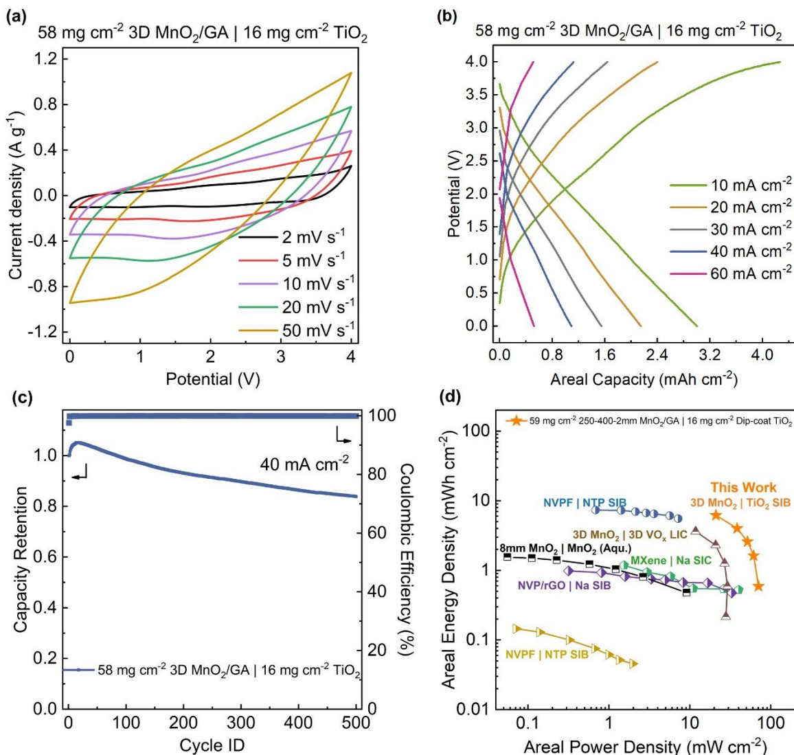
Figure 6. (a) The CV curve for a sodium ion battery device with 58 mg cm -2 3D MnO 2 /GA as cathode and 16 mg cm -2 dip-coated TiO 2 as anode from scan rate of 2 mV s -1 to 50 mV s -1 . (b) The GV curve for a sodium ion battery device with 58 mg cm -2 3D MnO 2 /GA as cathode and 16 mg cm -2 dip-coated TiO 2 as anode from 10 mA cm -2 to 60 mA cm -2 . (c) The long-term cycling performance of 3D MnO 2 | TiO 2 device at 40 mA cm -2 for 500 cycles. (d) The Ragone plot of areal energy density versus areal power density of 3D MnO 2 | TiO 2 device and the performance comparison with reported lithium-ion batteries and sodium-ion batteries devices with 3D electrodes.
