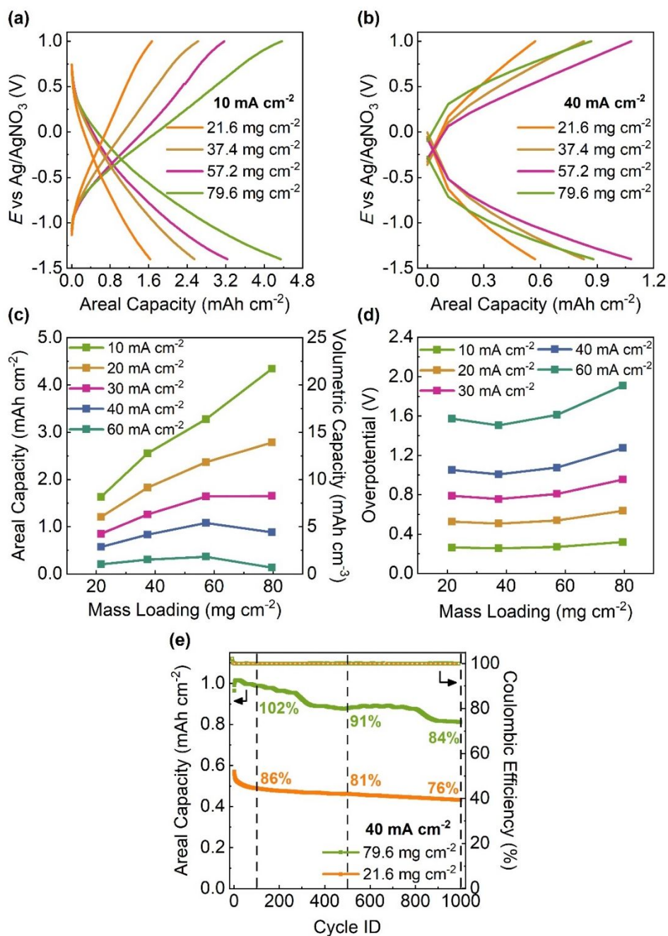
Figure 5. (a) The GV curves of 21.6, 37.4, 57.2, and 79.6 mg cm -2 MnO 2 /GA electrodes at a current density of 10 mA cm -2 . (b) The GV curves of 21.6, 37.4, 57.2, and 79.6 mg cm -2 MnO 2 /GA electrodes at a current density of 40 mA cm -2 . (c) The areal capacity and volumetric capacity of MnO 2 /GA at current densities from 10 mA cm -2 to 60 mA cm -2 for 21.6, 37.4, 57.2, and 79.6 mg cm -2 MnO 2 /GA electrodes. (d) The overpotentials at current densities from 10 mA cm -2 to 60 mA cm -2 for 21.6, 37.4, 57.2, and 79.6 mg cm -2 MnO 2 /GA electrodes. (e) The long-term cycling performance of 21.6 and 79.6 mg cm -2 MnO 2 /GA electrodes at a current density of 40 mA cm -2 for 1000 cycles.
