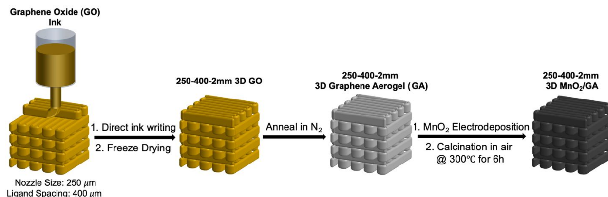
Figure 2. The schematic illustration of the preparation process of 250-400-2mm 3D \text{MnO}_2/\text{GA} electrode.
