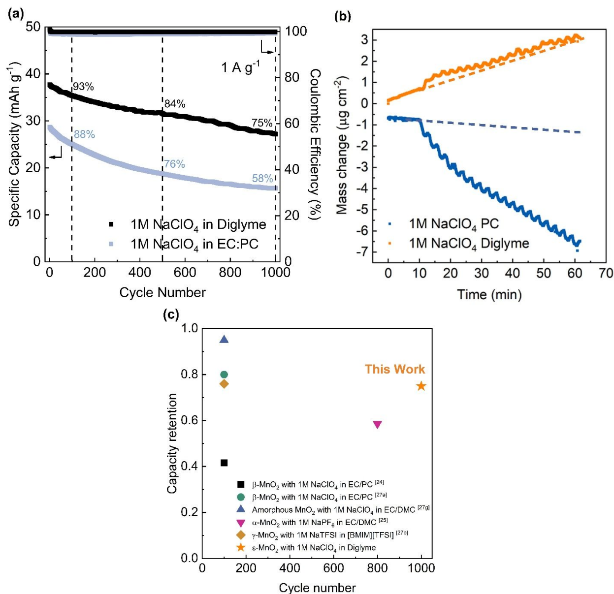
Figure 1. (a) The long-term cycling stability comparison of \text{MnO}_2 in 1M \text{NaClO}_4 in diglyme and 1M \text{NaClO}_4 in EC/PC electrolyte. (b) EQCM results showing the mass change for \text{MnO}_2 in diglyme and PC electrolyte during OCV (initial 10 minutes) and during CV measurements. The diglyme electrolyte shows effectively no mass change (except baseline mass change) while the PC electrolyte exhibits a continuous decrease in mass. (c) Capacity retention as a function of cycling for \text{MnO}_2 in various electrolytes.
