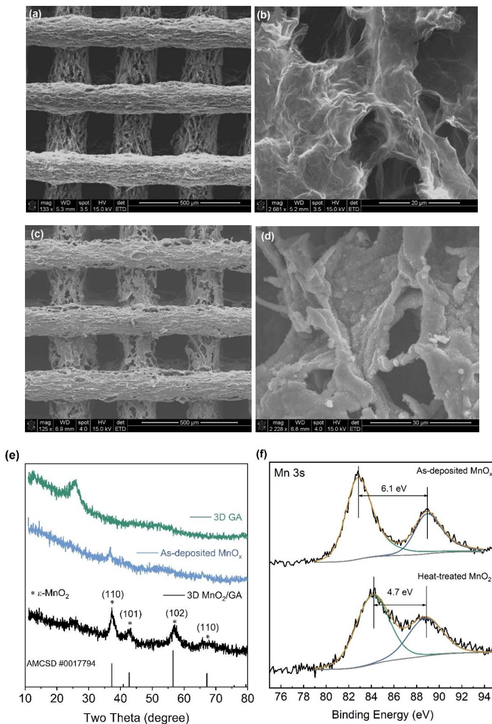
Figure 3. (a), (b) The planar view SEM image of pure 3D GA. (c), (d) The planar view SEM image of 21.6 mg cm -2 MnO 2 /GA and morphology of deposited MnO 2 . (e) The XRD patterns of 3D GA, as-deposited MnO x , 3D MnO 2 /GA after heat treatment and the standard XRD pattern (AMCSD #0017794) of ε-MnO 2 . (f) The XPS spectra of Mn 3s for as-deposited MnO x and 3D MnO 2 /GA.
