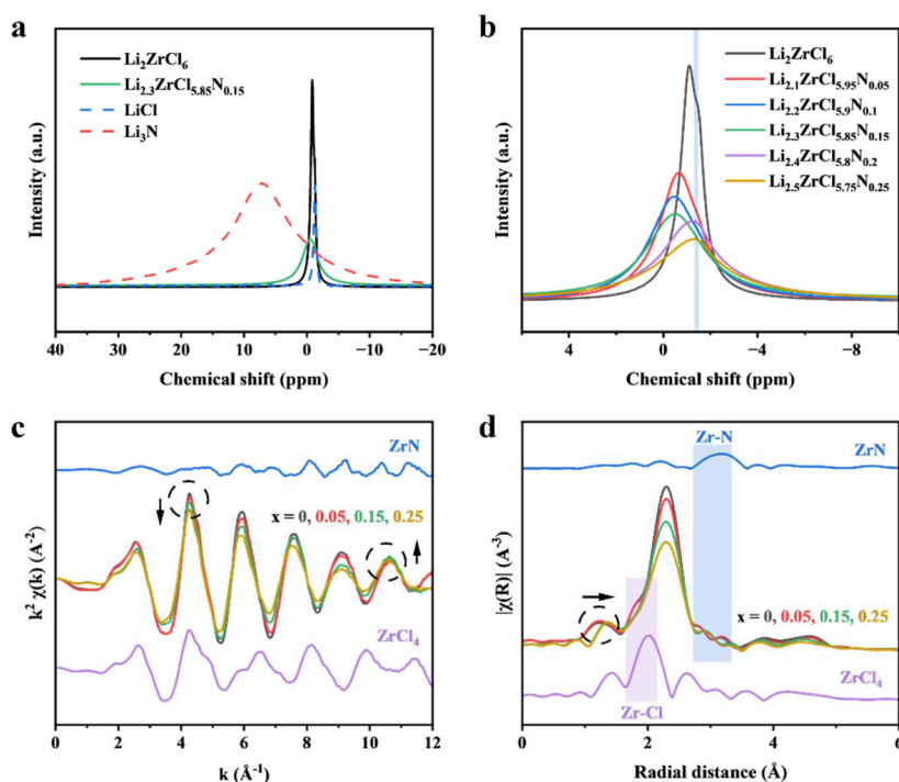
Fig. 2 (a) The ^7\text{Li} ssNMR spectra of LZC, LZC-N0.15, LiCl, and \text{Li}_3\text{N} . (b) Evolution of ^7\text{Li} ssNMR spectral features in LZC-N x with increasing N-doping levels. (c) K -space and (d) R -space of the XAS spectra of LZC, LZC-N0.05, LZC-N0.15, LZC-N0.25, ZrN, and \text{ZrCl}_4 .
