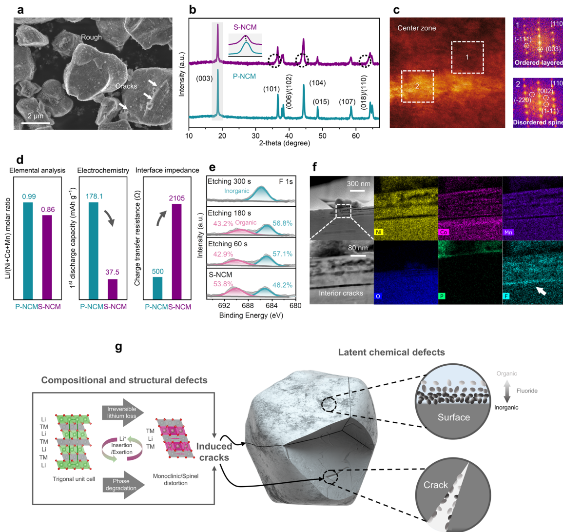
Fig. 1 Neglected chemical residuals on the 250k-miles-served cathode. (a) SEM image and (b) XRD pattern of the degraded S-NCM. The black dotted circle accentuates the subtle peaks that do not belong to the layered structure; (c) high-resolution HAADF-STEM images on the central area of the S-NCM particle and the FFT patterns of the selected dark and bright regions; (d) comprehensive comparison of lithium loss in degraded powders measured by ICP-OES, electrochemical capacity, and charge-transfer resistance analyses in the half-cell using S-NCM and P-NCM powders as cathode active materials; (e) F 1s XPS patterns of S-NCM powders for different sputtering times using an ion-beam. Based on the calculated integral area, the proportional values of the organics and inorganics in fluoride are presented in the patterns; (f) HAADF-STEM images based on focused ion beam cutting and an enlarged view displaying the interior microcracks. Corresponding EDS mapping analysis indicates the presence of F element along these microcracks pointed out by a white arrow. (g) Deficiencies of S-NCM addressed before direct regeneration, including the compositional and structural aspects (e.g., irreversible lithium-ionic loss, phase degradation, internal and external cracks) and latent chemical defects (e.g., surface and crack-edge impurities enriching the F element).
