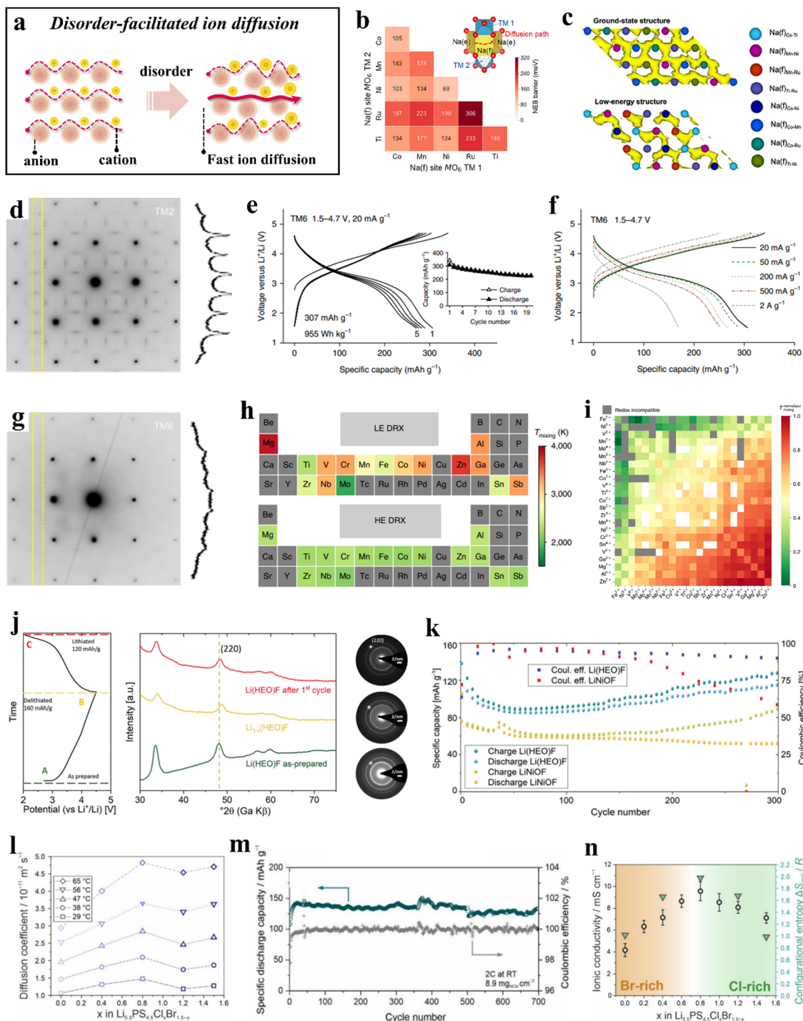
Fig. 7 (a) Schematic illustration of disorder-facilitated ion diffusion. (b) and (c) Theoretical calculations for P2-TMCNR. 273 (b) Na + migration barriers of different Na(f) M TM 1 . (c) AIMD trajectories for the ground-state structure and a low-energy structure. (d)–(i) DRX compounds. 211 (d) ED pattern collected from TM2 along the [100] zone axis. (e) Voltage profiles of TM6 within the potential window of 1.5–4.7 V at 20 mA g -1 . (f) Rate capability of TM6. (g) ED pattern collected from TM6 along the [100] zone axis. (h) Periodic table-type heat map of mixing temperatures of different elements in LE and HE DRXs. (i) Normalized mixing temperatures. (j) and (k) Li(HEO)F and LiNiOF cathodes. 276 (j) Initial charge/discharge curve at C/10 (20 mA g -1 ) in the potential range between 2.0 and 4.5 V (left) and the corresponding ex situ XRD patterns (middle), as well as ED data (right). (k) Comparison of capacity retentions at C/10 of Li(HEO)F and LiNiOF. (l)–(n) Li 5.5 PS 4.5 Cl x Br 1.5-x electrolytes. 274 (l) Lithium-diffusion coefficients at different temperatures. (m) Capacity retention and Coulomb efficiencies. (n) Ionic conductivity as a function of x.
