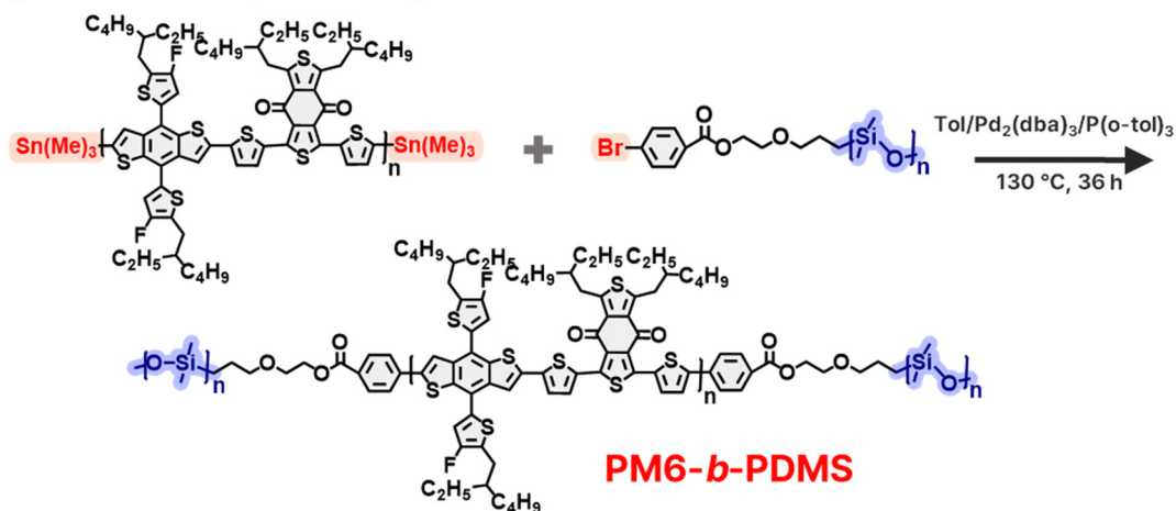
Scheme 1 Synthetic schemes of (a) \text{PM6-}b\text{-PDMS} and (b) DYPDMS.
