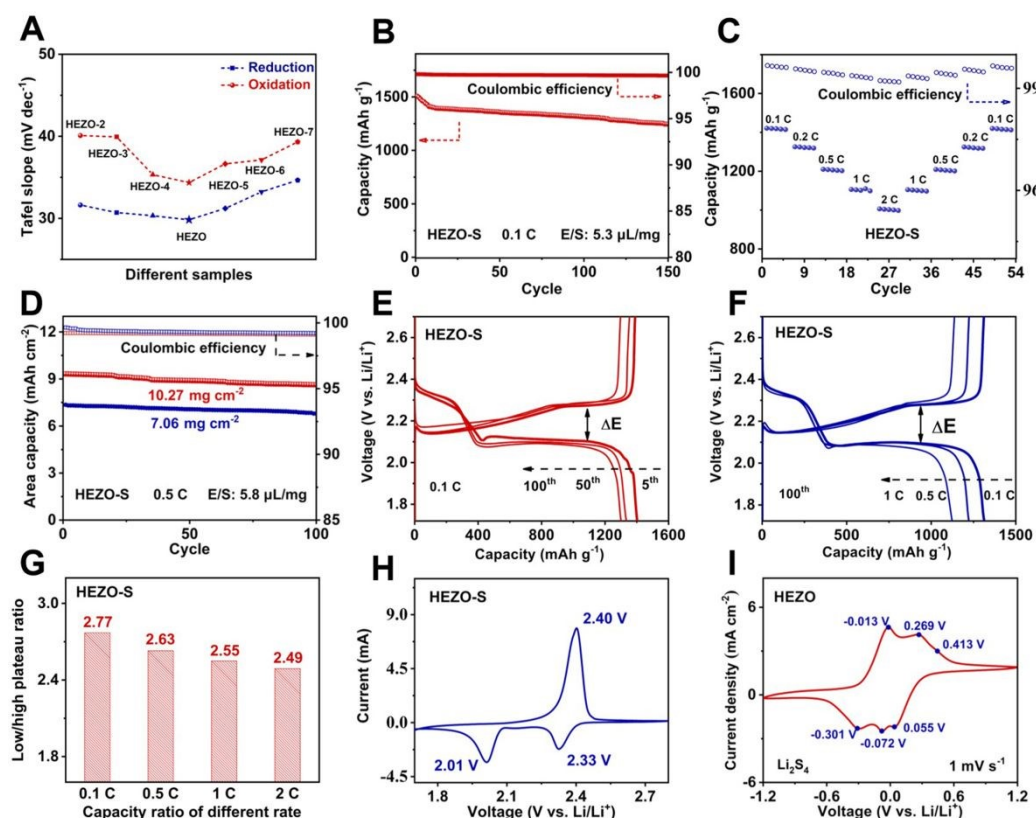
Fig. 3 | Electrochemical performance of HEZO-S cathode. A , Tafel slopes of different HEZO components. B , Long-cycling performance at 0.1 C. C , Rate capabilities from 0.1 C to 2 C. D , Long-cycling performance with different sulfur loading at 0.5 C. E , Galvanostatic discharge-charge curves of different cycle numbers at 0.1 C. F , Galvanostatic discharge-charge curves of different current densities at 100th cycle. G , Ratio of low to high platform capacity under different rates. H , CV curves of HEZO-S normal cell and I , HEZO- \text{Li}_2\text{S}_6 catholyte symmetric cell.
