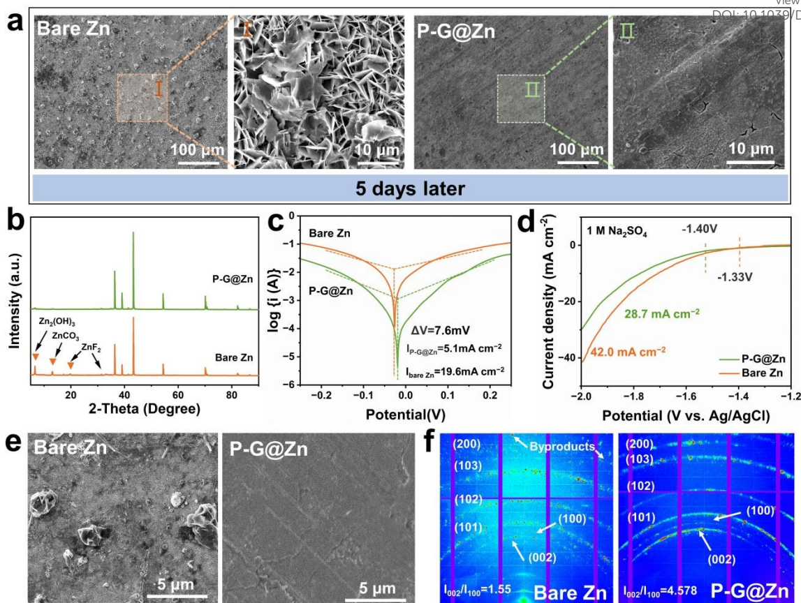
Fig. 2. Anti-corrosion performance of P-G@Zn anode. (a) Surface SEM images of bare Zn and P-G@Zn immersed in electrolyte after 5 days. (b) XRD patterns of bare Zn and P-G@Zn soaked in electrolyte after 5 days. (c) Tafel curves of bare Zn and P-G@Zn. (d) LSV curves of bare Zn and P-G@Zn. (e) SEM images of bare Zn and P-G@Zn after removing the P-G layer after cycling 60 h at 1 mA cm -2 . (f) WAXS patterns for cycled bare Zn and cycled P-G@Zn.
