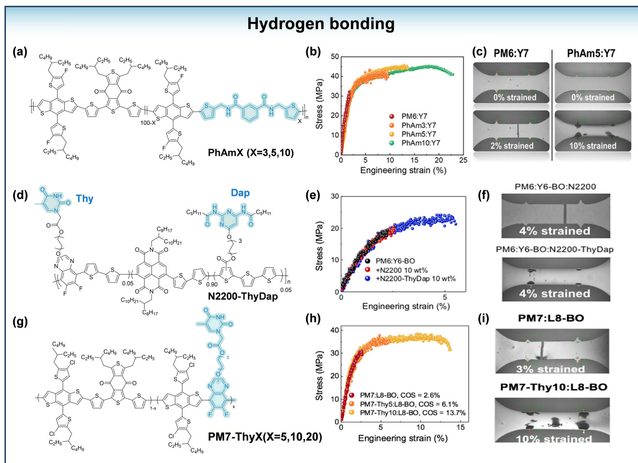
Fig. 7 (a) The chemical structure of PhAmX (X = 3, 5, 10). (b) The stress–strain curves of the blend films of PM6:Y7, PhAm3:Y7, PhAm5:Y7 and PhAm10:Y7. (c) Images of blend films during the tensile test. (d) The chemical structure of N2200-ThyDap. (e) The stress–strain curves of the blend films of PM6:Y6-BO, PM6:Y6-BO:N2200 and PM6:Y6-BO:N2200-ThyDap (wt% value of P_A indicates the weight of P_A compared to ( P_A + SMA) weight). (f) Images of blend films during the tensile test. (g) The chemical structure of PM7-ThyX (X = 5, 10, 20). (h) The stress–strain curves of the blend films of PM7:L8-BO, PM7-Thy5:L8BO, and PM7-Thy10:L8-BO. (i) Images of blend films during the tensile test. (b) and (c) Reproduced with permission from ref. 59. Copyright 2022, Wiley-VCH. (e) and (f) Reproduced with permission from ref. 60. Copyright 2023, American Chemical Society. (h) and (i) Reproduced with permission from ref. 62. Copyright 2023, American Chemical Society.
