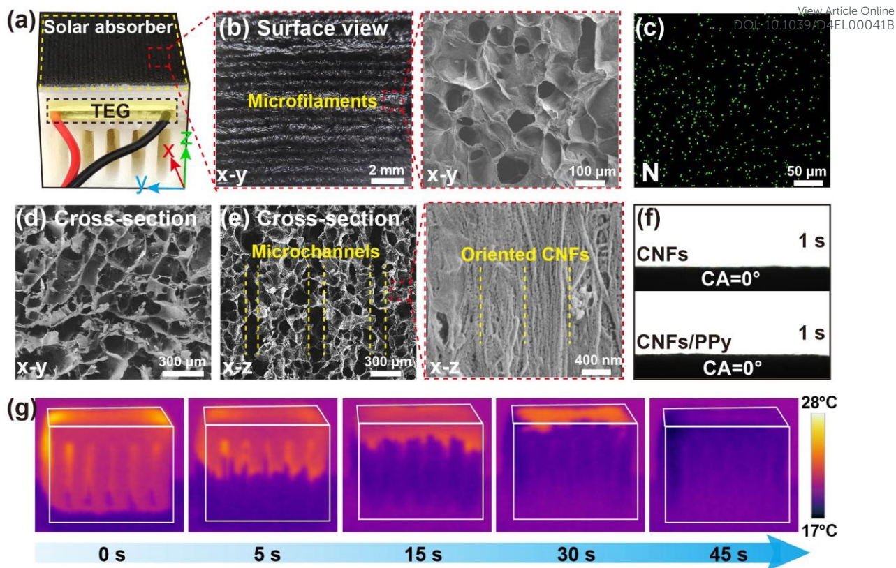
Fig. 3 (a) Digital photograph of heatsink-like SG-TEG hybrid device. (b) Surface macro photography (left) and a local SEM image (right). (c) EDS image of the characteristic element. (d) SEM images of the transverse cross-sections. (e) SEM images of the longitudinal cross-sections. (f) Surface contact angle measurements. (g) Water diffusion characterization over 45 s.
