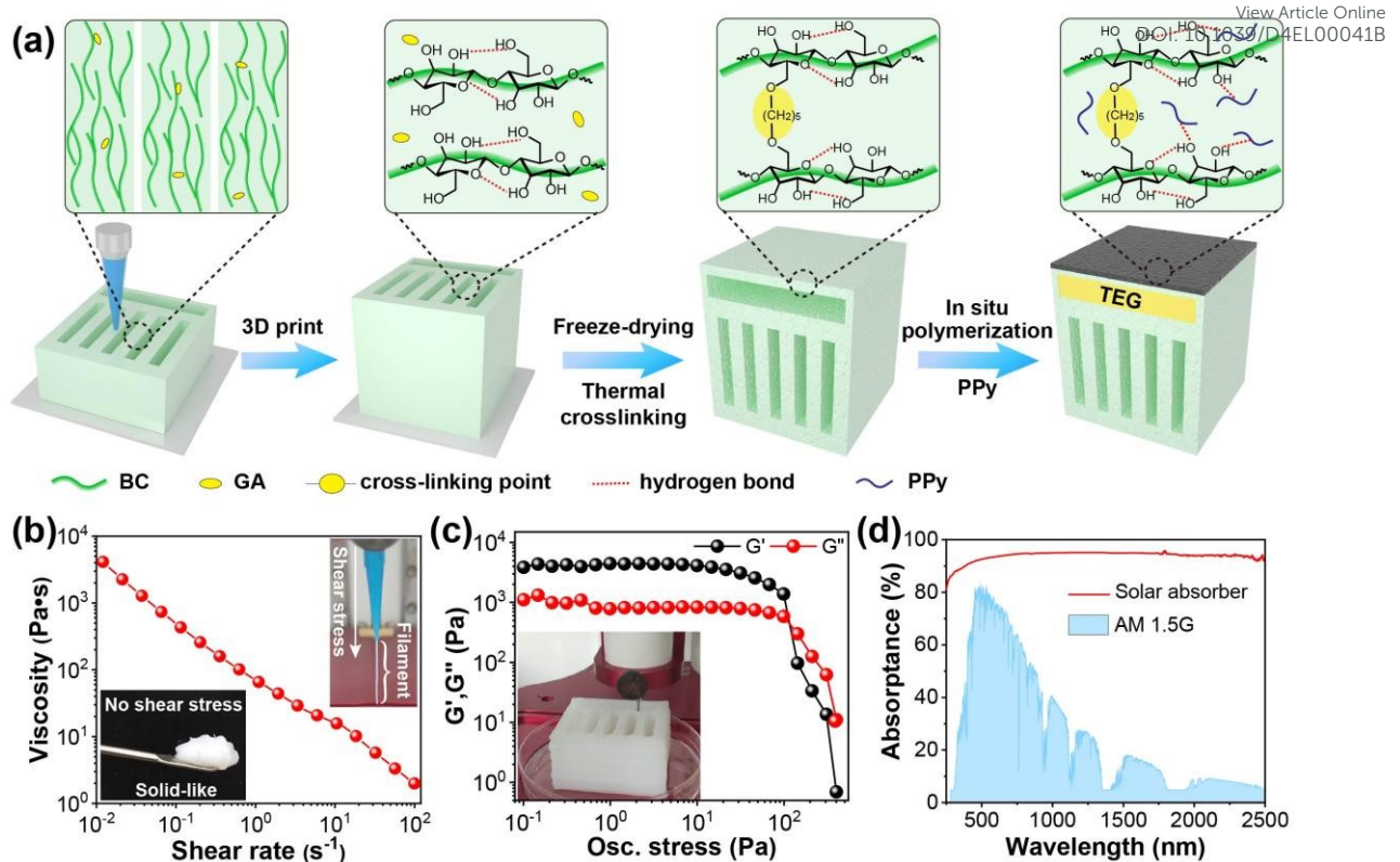
Fig. 2 (a) A flow chart of the fabrication of heatsink-like SG-TEG hybrid device. (b) Shear viscosity of the printing ink under shear rate sweep (The insert images show the printing inks with and without shear stress). (c) Rheological properties of the printing ink: G' and G'' under oscillation stress sweep (The insert image shows the 3D printed model). (d) An absorbance spectrum of CNFs/PPy composite aerogel.
