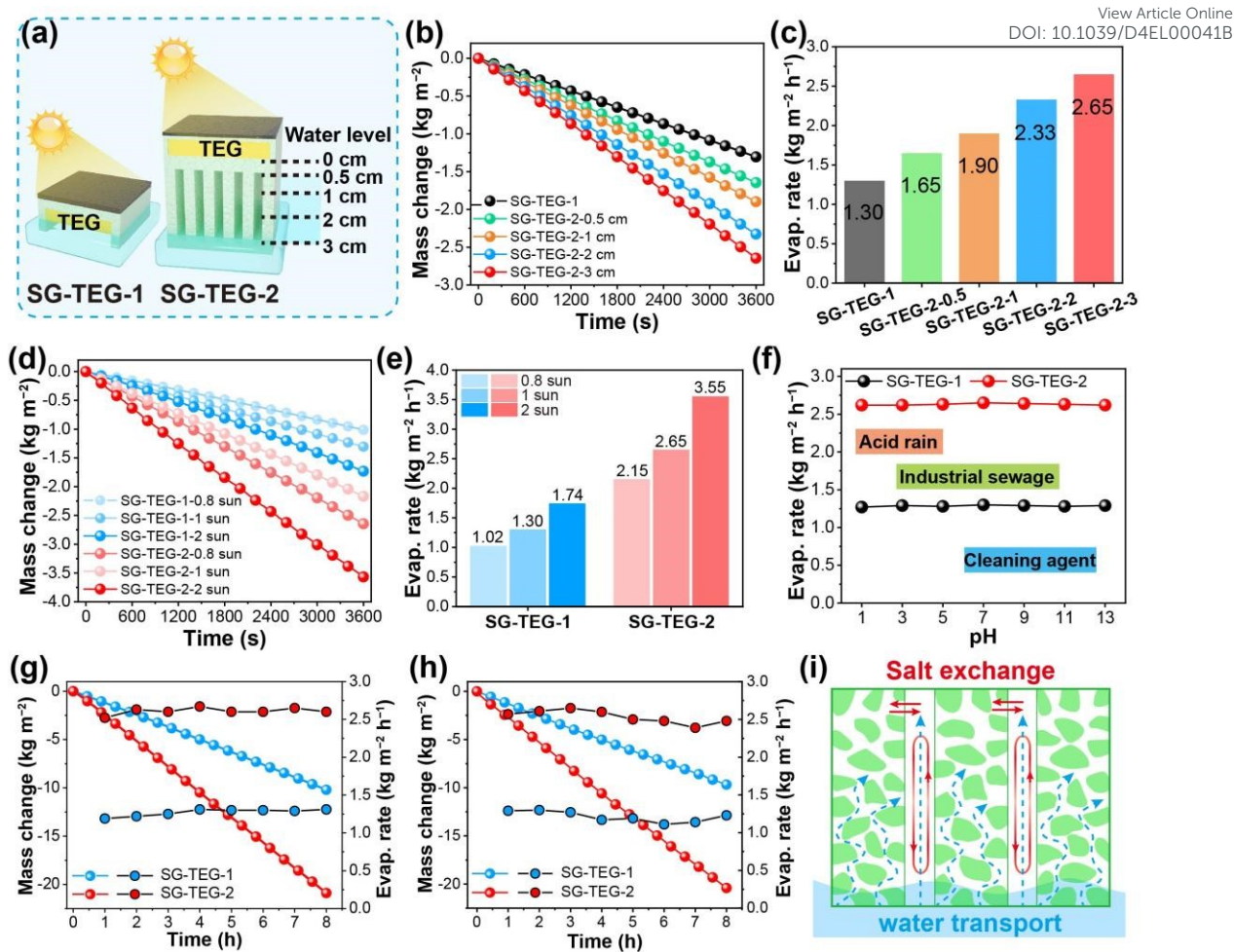
Fig. 4 (a) Schematic illustration of SG-TEG-1 and SG-TEG-2. (b) Mass changes and (c) summary of water evaporation rates under 1 sun. (d) Mass changes and (e) summary of water evaporation rates under different solar irradiation. (f) Water evaporation rates of SG-TEG-1 and SG-TEG-2 in a wide range of pH. Solar desalination of SG-TEG-1 and SG-TEG-2 in (g) 3.5 wt.% and (h) 10 wt.% brine. (i) Schematic illustration of the salt-exchange mechanism.
