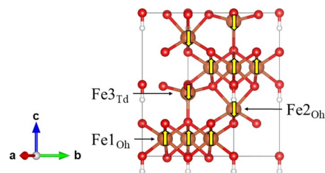
Fig. 1 Ferrimagnetic Fh bulk unit cell. The six Fe1 Oh sites are spin-up and two Fe2 Oh and two Fe3 Td sites are spin-down as per Pinney's ferrimagnetic arrangement. Colour scheme: Fe, orange; O, red; H, white.
