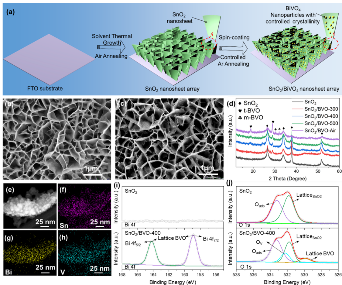
Fig. 1 (a) Schematic synthesis procedure of the \text{SnO}_2/\text{BVO} nanosheet array photoanode; (b) and (c) SEM images of the pristine \text{SnO}_2 nanosheet array and the \text{SnO}_2/\text{BVO-400} heterostructure nanosheet array. (d) XRD pattern of pristine \text{SnO}_2 and \text{SnO}_2/\text{BVO} samples under different annealing conditions. (e) HAADF-STEM image of \text{SnO}_2/\text{BVO-400} , (f)–(h) Sn, Bi, V EDS-mapping images of \text{SnO}_2/\text{BVO-400} . (i) and (j) High-resolution Bi 4f and O 1s XPS spectra of pristine \text{SnO}_2 and \text{SnO}_2/\text{BVO-400} .
