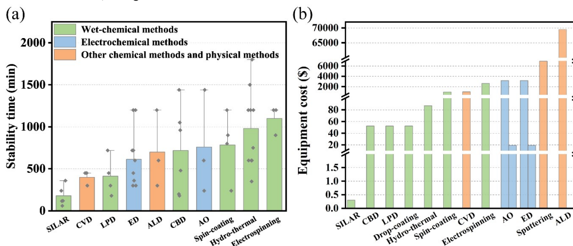
Fig. 3. (a) The stability duration of the photoanodes prepared by different methods was counted from the literature. Based on the cycling experiments or photocurrent-time curves mentioned in the literature, the total number of minutes of stability tests carried out is considered to be the stable duration of the photoanode if there is no significant decrease in activity during the test period (Drop-coating and sputtering methods are not shown because there are fewer than three references). (b) The cost of equipment required to prepare non-TiO 2 -based photoanodes. AO (anodic oxidation) and ED (electrochemical deposition) can be operated using an electrochemical workstation and a DC power supply, so there are two prices for them. The price of the equipment is from www.1688.com, and the lowest price of the same type of product is selected for comparison.
