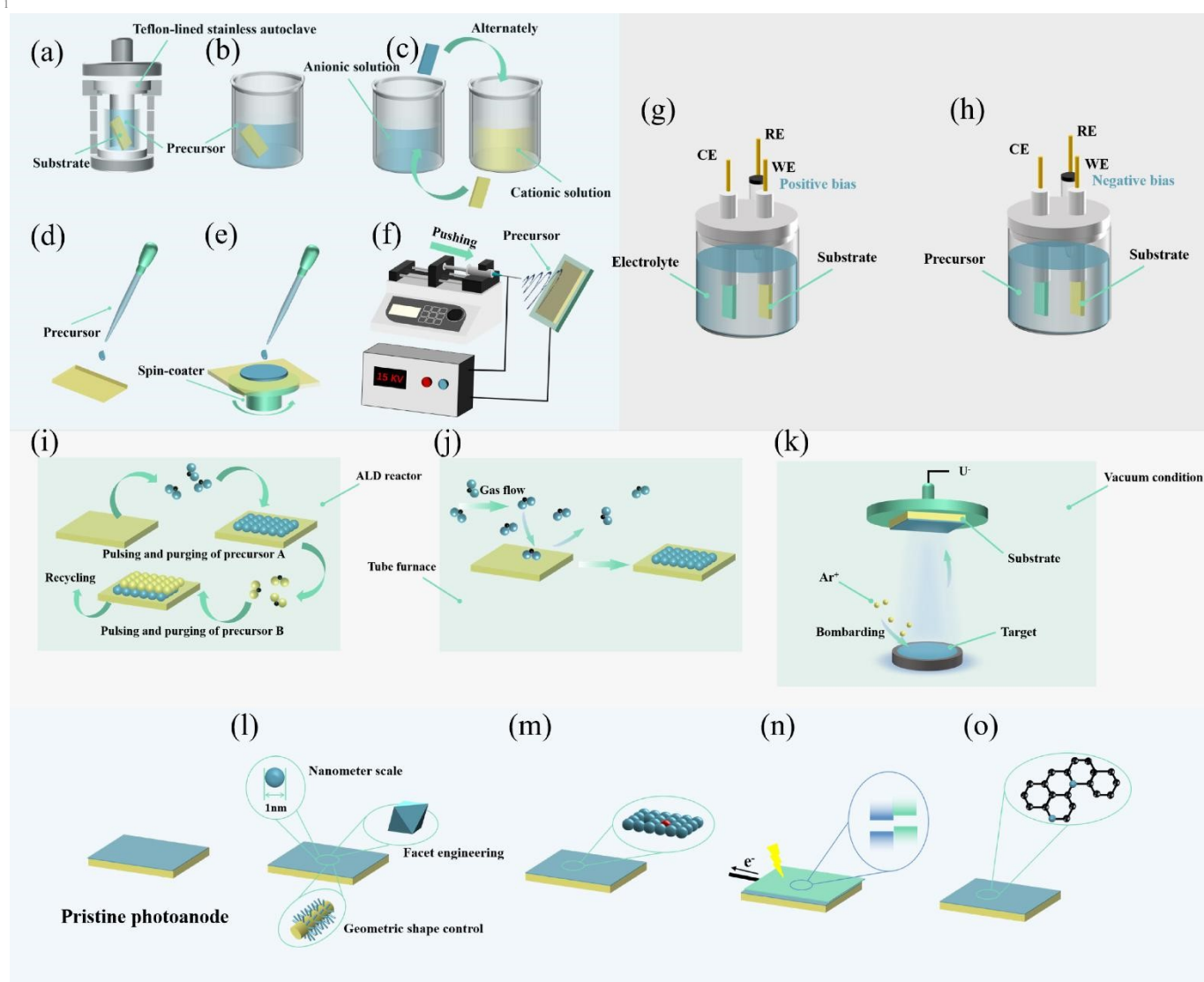
Fig. 4. Synthesis and modification methods for non-TiO 2 -based photoanodes. Wet-chemical methods: (a) hydrothermal method; (b) CBD and LPD; (c) SILAR; (d) drop-coating; (e) spin-coating; (f) electrospinning. Electrochemical methods: (g) anodic oxidation and (h) electrochemical deposition. Other chemical methods: (i) ALD and (j) CVD. Physical methods: (k) sputtering. Modification methods: (l) morphological modification; (m) doping modification; (n) heterojunction; (o) combining with co-catalysts.
