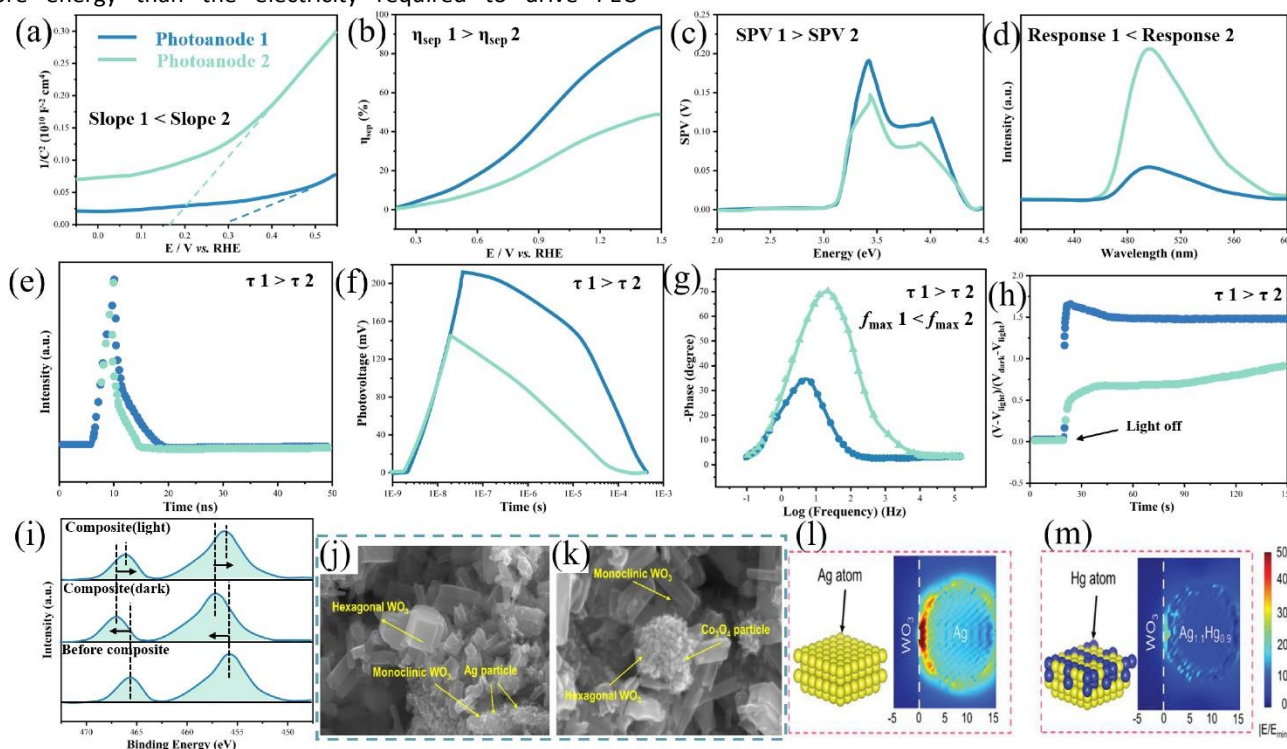
Fig. 7. Techniques used to characterize separation efficiency: Schematic diagram of (a) Mott-Schottky plot, (b) charge separation efficiency, (c) steady-state SPV results, and (d) steady-state PL spectra (where it is assumed that the separation efficiency of Photoanode 1 is higher than that of Photoanode 2); Charge transfer kinetics: Schematic diagram of (e) TRPL decay spectra, (f) transient photovoltage result, (g) Bode plot, and (h) normalized OCP decay curves (where it is assumed that Photoanode 1 has a longer decay lifetime than Photoanode 2); Charge transfer pathway: (i) Schematic XPS spectra of the composite photoanode in different conditions, (j-k): SEM images of WO 3 photoanode after photochemical deposition of Ag and Co 3 O 4 , reprinted from ref. 46, Copyright (2022), with permission from Elsevier. (l-m): DDA simulations for the electric field intensity at the WO 3 nanoplate and Ag nanocrystal interface before and after Hg 2+ pretreatment, reprinted with permission from ref. 51 Copyright (2023) Wiley-VCH.
