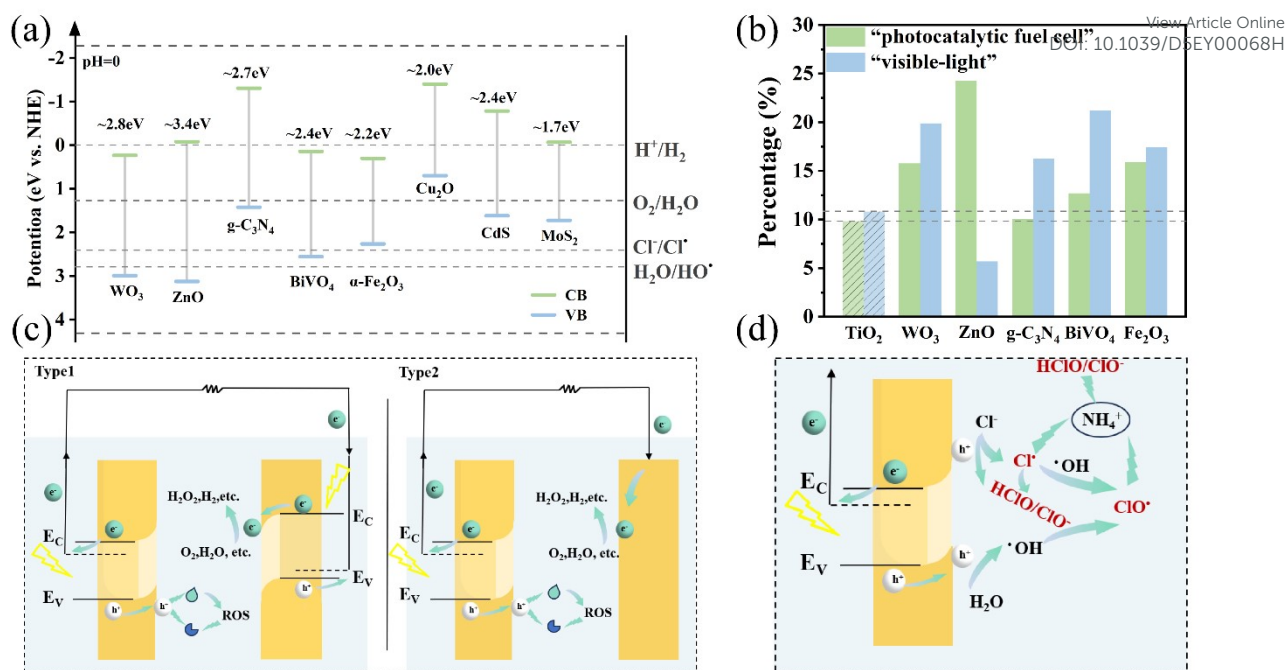
Fig. 2. (a) The band structures of eight main non-TiO 2 -based photoanodes. Data from ref. 33-36. (b) Bibliometric analysis of TiO 2 and the five most frequently used non-TiO 2 -based photoanodes. (Counting the keywords in the titles of the literature, filtering out words like 'and', 'of', 'degradation', and 'photoanode' that do not reflect the key information, and the most significant remaining keywords are "fuel cell", "visible-light", and the proportion of the literature containing these keywords to the total literature was calculated). (c) The schematic of two types of PFC with non-TiO 2 -based photoanodes. (d) A schematic diagram of the possible sources of RCS generation in the PEC-Cl system. 34
