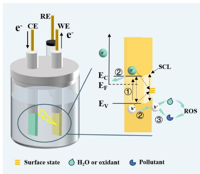
Scheme 1. Schematic diagram of the process around the photoanode for PEC wastewater treatment (n-type semiconductor as an example). CE: counter electrode, RE: reference electrode, WE: working electrode, E_C : conduction band potential, E_F : Fermi energy level, E_V : valence band potential, SCL: space charge layer, ROS: reactive oxygen species.
