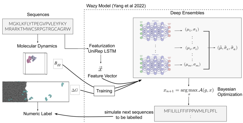
Fig. 1 Schematic overview of the active learning framework for predicting peptides using Bayesian Optimisation (BO) and Molecular Dynamics (MD) simulations: (A) MD simulations of protein chains to compute second virial coefficient ( B_{22} ) and partition free energy ( \Delta G ) for model training. This initial sample is fed to the wazy BO package, 25 which utilises UniRep LSTM, 24,26 to parse the protein sequence into a feature vector \vec{x} . Deep ensemble training on feature vectors and computed properties to establish sequence–property relationships. To choose which sequences the model would benefit the most from, an acquisition function \mathcal{A} is used to rank and suggest the next set of sequences. The suggested sequences are simulated again, generating new data for subsequent training cycles. This iterative process helps the model learn the sequence–property relationship with fewer examples and simultaneously explore sequence space regions that contain proteins with the most extreme values of the property we studied.
