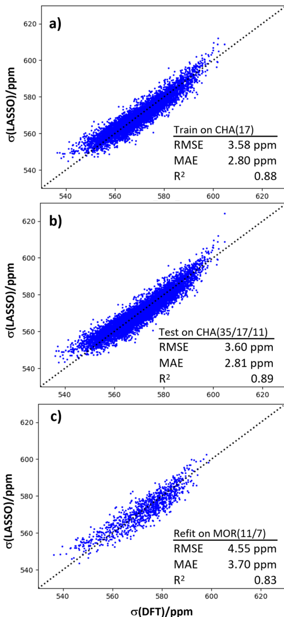
Fig. 6 (a) Validation of the LASSO regression model against the training set of ^{23}\text{Na} chemical shifts of CHA(17) configurations. (b) Generalization test of the LASSO model against CHA(35) and CHA(11) configurations. (c) Performance of the refitted model against MOR(11) data.
