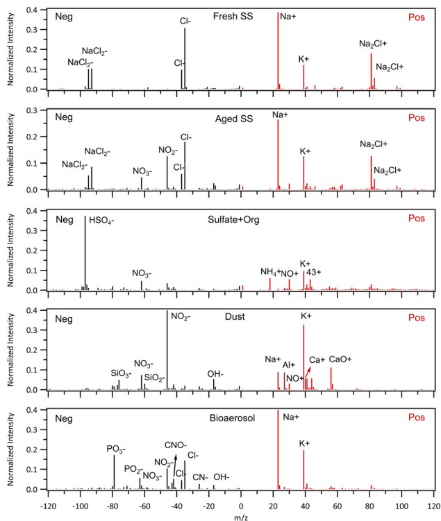
Fig. 5 Average spectra of (from the top to bottom) fresh sea salt, aged sea salt, sulfates, dust, and bioaerosol, from aerosol sampling. It is noted that only one spectrum of bio-aerosol in aerosol mode was detected.
