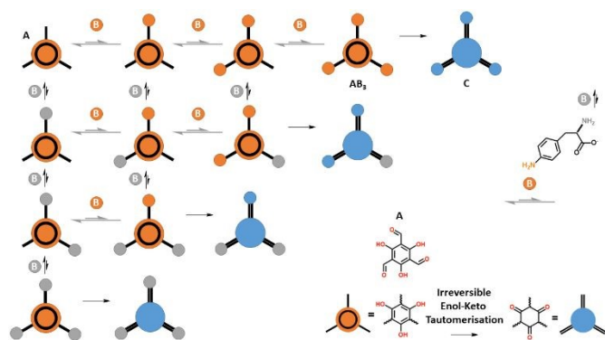
Figure 2. Reaction Network showing the thirteen possible products from the mixing of A (1,3,5-triformylglucinol) and B (4-amino- L -phenylalanine) in water at a pH of approximately 8. A can react with B through the aniline functional group (horizontal equilibrium arrows (orange)) or the alkyl amine functional group (vertical equilibrium arrows (grey)). Both equilibria are biased towards starting materials due to water. The irreversible enol-keto tautomerisation only occurs once all three aldehyde functional groups have reacted, shown as a horizontal reaction unidirectional arrow. Only the product C is analytically observed. It results from the tautomerisation of AB 3 (the thrice reacted aniline product).
