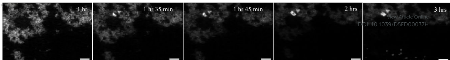
Figure 5 \text{Ca-K}\alpha fluorescence maps extracted from n -XRF spectra at different time points during in situ \text{CaP} crystallisation in a liquid cell. scale bar = 500nm
