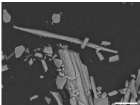
Figure 7 SEM image of calcite prisms from M. edulis after dissolution of interprismatic organic matrix. Scale bar 10 \mu\text{m}
