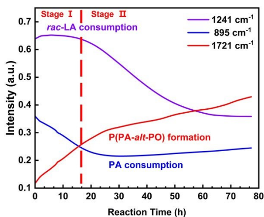
Fig. 5 Time-resolved in situ IR spectra during the polymerization of mixtures of PA, PO, and rac -LA. Reaction conditions: CHD/(S,S)-TUC/PA/PO/ rac -LA = 1/5/100/200/200, 80 °C, and toluene as the solvent.
