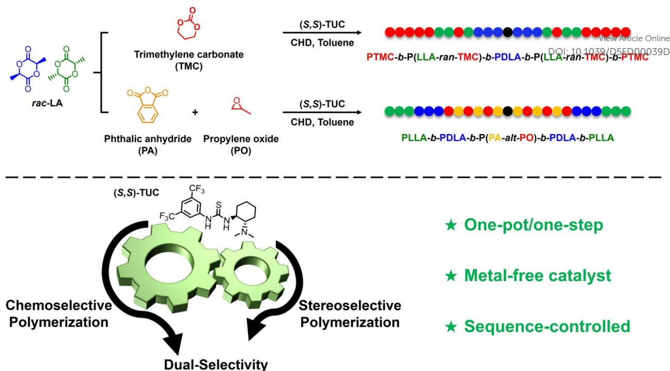
Scheme 1 Chemoselective and stereoselective ring-opening polymerization of mixed epoxides, cyclic anhydrides, cyclic carbonates and cyclic esters using (S,S)-TUC as the catalyst.
