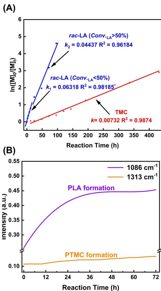
Fig. 2 (A) The kinetic curves for the ring-opening copolymerization of rac -LA and TMC. Reaction conditions: CHD/[( S,S )-TUC]/ rac -LA/TMC = 1/5/50/50, at 40 °C, in toluene. (B) Time resolved in situ IR spectra during the polymerization of mixtures of rac -LA and TMC. Reaction conditions: CHD/[( S,S )-TUC]/ rac -LA/TMC = 1/5/50/50, 40 °C, in toluene.
