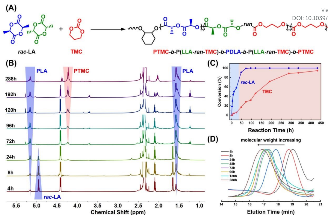
Fig. 1 (A) Scheme of the ring-opening copolymerization mechanism of rac -LA and TMC by using (S,S)-TUC as catalyst. (B) The 1 H NMR spectra of crude aliquots taken from the reaction system for monitoring the conversion of rac -LA and TMC and the formation of the block copolymer PTMC- b -P(LLA- ran -TMC)- b -PDLA- b -P(LLA- ran -TMC)- b -PTMC in CDCl 3 . (C) Time-dependent plots of monomer conversion rates, determined from 1 H NMR spectra. (D) SEC traces at different reaction time.
