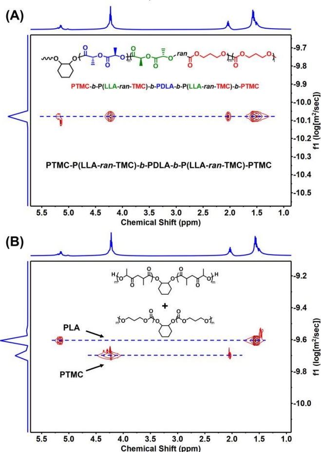
Fig. 4 1 H NMR DOSY spectra of (A) PTMC- b -P(LLA- ran -TMC)- b -PDLA- b -P(LLA- ran -TMC)- b -PTMC and (B) a blend of PLA and PTMC homopolymer, in CDCl 3 , respectively.
