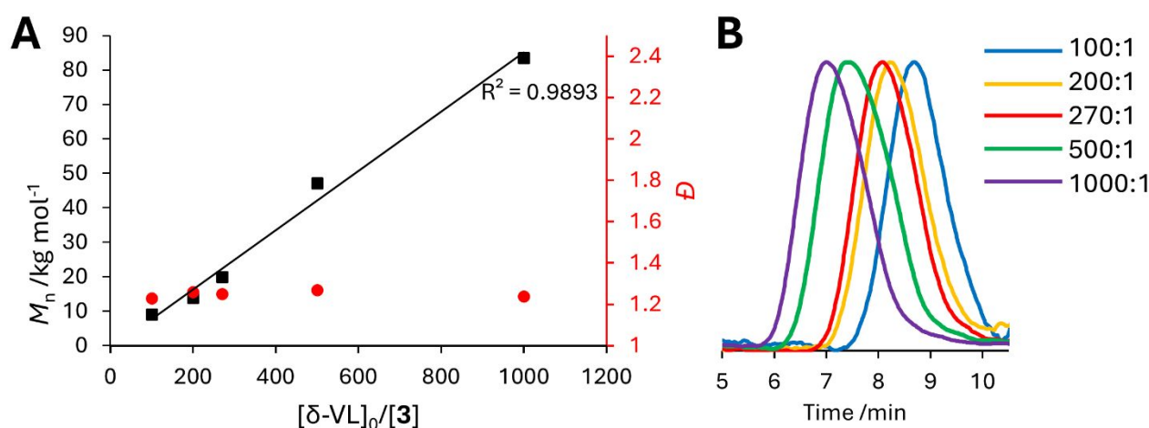
Figure 2: (A) Plot showing the relationship between M_n of PVL (black squares) and \bar{D} (red circles) with varying [\delta\text{-VL}]_0/[\mathbf{3}] ; (B) GPC traces of PVL at various [\delta\text{-VL}]_0/[\mathbf{3}] ratios.
