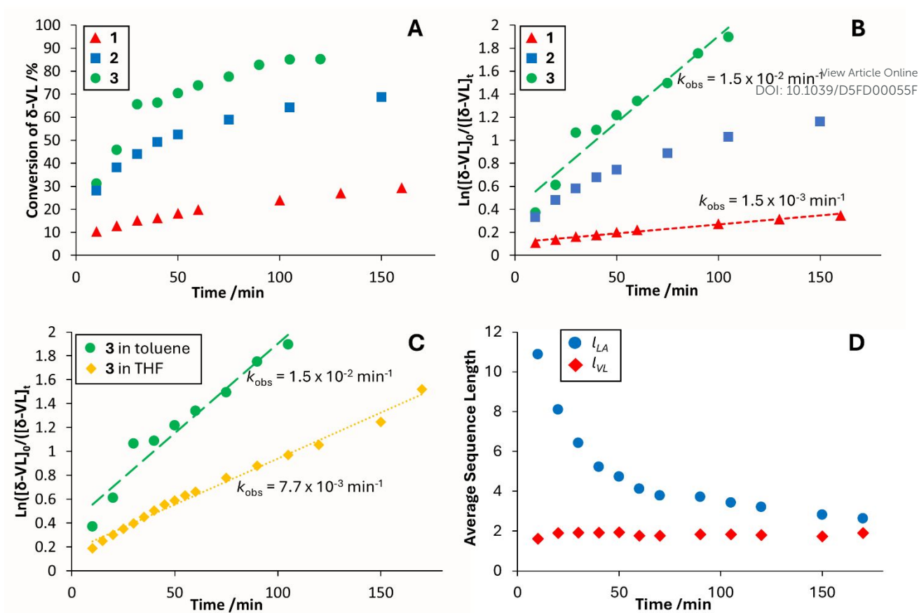
Figure 8: (A) Plot showing percentage conversion of \delta -VL with time ( rac -LA conversion is at >99% after 5 min) using 1 (red triangle), 2 (blue square) and 3 (green circle) in toluene; (B) Semi-logarithmic plot for \delta -VL polymerisation using 1 (red triangle), 2 (blue square) and 3 (green circle) in toluene; (C) Semi-logarithmic plot for \delta -VL polymerisation using 3 in toluene (green circle) and THF (yellow diamond); (D) Average sequence length of LA (blue circle) and VL (red diamond) units over time in poly(lactide-co-valerolactone) prepared using 3 in THF. Reaction conditions: [\text{rac-LA}]_0 = [\delta\text{-VL}]_0 = 0.5 \text{ M} at ambient temperature, [M]_0/[La] = 200 .
