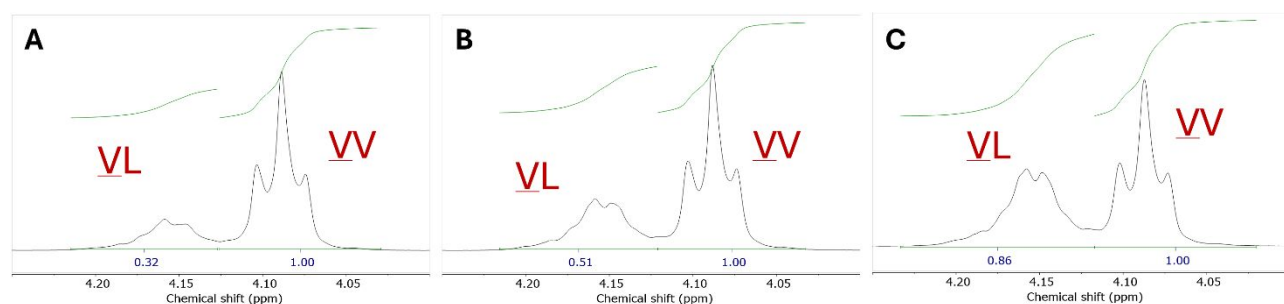
Figure 5: Comparison of the relative integration of the signals assigned to VL and VV diads in the ^1\text{H} NMR spectra of poly(lactide-co-valerolactone) copolymers prepared using: (A) 2 in toluene (table 2, entry 9), (B) 3 in toluene (table 2, entry 11), (C) 3 in THF (table 2, entry 12).
