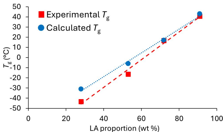
Figure 7: Plot showing experimental and calculated T_g for poly(lactide-co-valerolactone)s prepared using 3 at variable monomer feed ratios.
