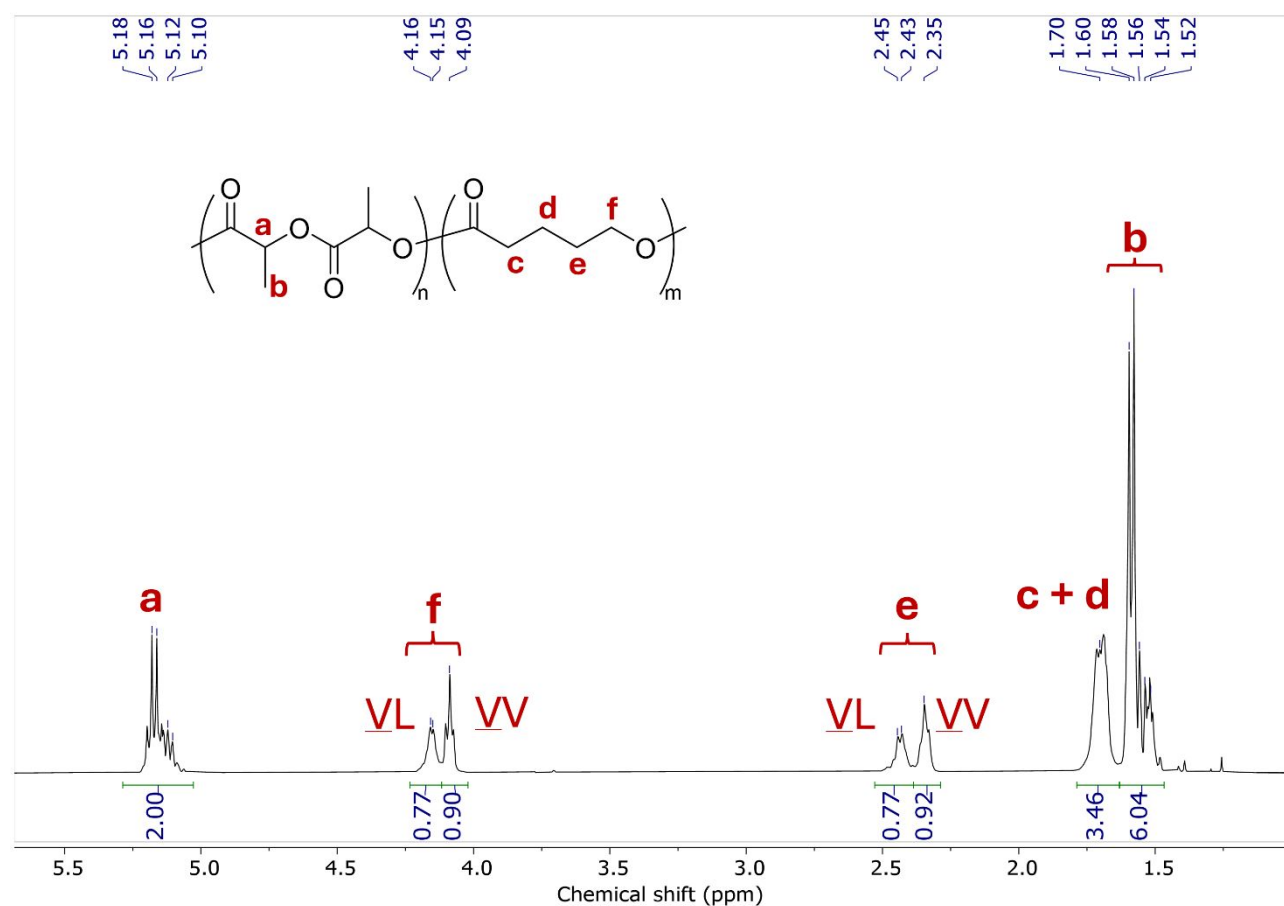
Figure 4: Assignment of the ^1\text{H} NMR spectrum of poly(lactide-co-valerolactone) copolymer prepared using 3 (Table 2, entry 12). V = valeroyl unit ( -\text{C(O)}(\text{CH}_2)_4\text{O}- ), L = lactyl unit ( -\text{C(O)}(\text{CH}(\text{CH}_3)\text{O}- ), LL = lactidyl unit ( -\text{C(O)}(\text{CH}(\text{CH}_3)\text{OC(O)}(\text{CH}(\text{CH}_3)\text{O}- ).
