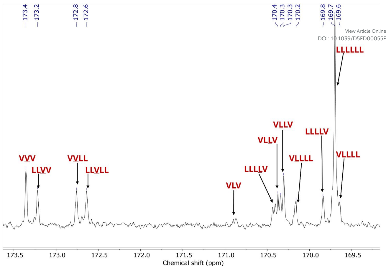
Figure 6: Carbonyl region in the quantitative ^{13}\text{C} NMR spectrum of a poly(lactide-co-valerolactone) prepared using 3 in THF (Table 2, entry 12). V = valeroyl unit ( -\text{C}(\text{O})(\text{CH}_2)_4\text{O}- ), L = lactyl unit ( -\text{C}(\text{O})(\text{CH}(\text{CH}_3)\text{O}- ), LL = lactidyl unit ( -\text{C}(\text{O})(\text{CH}(\text{CH}_3)\text{OC}(\text{O})(\text{CH}(\text{CH}_3)\text{O}- ).
