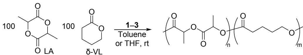
Scheme 2: Copolymerisation of LA and \delta -VL in toluene or THF catalysed by 1 – 3 .
