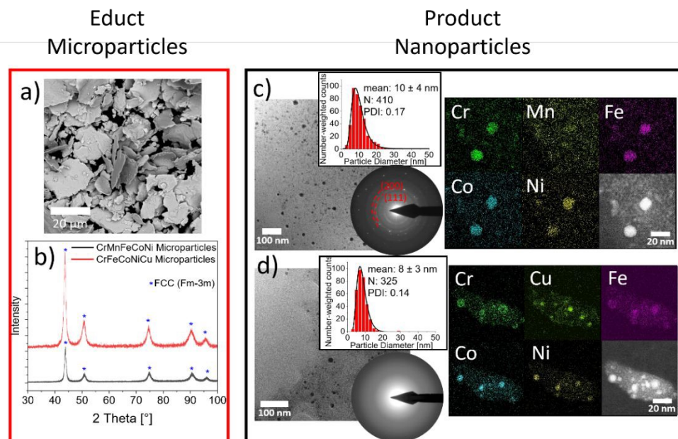
Figure 3. MP-LFL, conducted in ethanol for CrMnFeCoNi and CrFeCoNiCu MPs at a fluence of 1.8 \text{ J/cm}^2 , synthesizing HEA NPs via MP-LFL. Exemplary SEM image (a) and X-ray diffraction pattern (b) of the crystalline educt CrMnFeCoNi and CrFeCoNiCu MPs, showing a uniform fcc structure. TEM- and SAED images with corresponding particle size distribution are complemented by exemplary STEM-EDX maps of HEA NPs products generated via MP-LFL for CrMnFeCoNi (c) and CrFeCoNiCu (d), shows how composition sets partial segregation (Cr-Cu in Cu-containing HEA NPs) and structural development (crystalline Mn-containing HEA NPs and amorphous Cu-containing HEA NPs).
