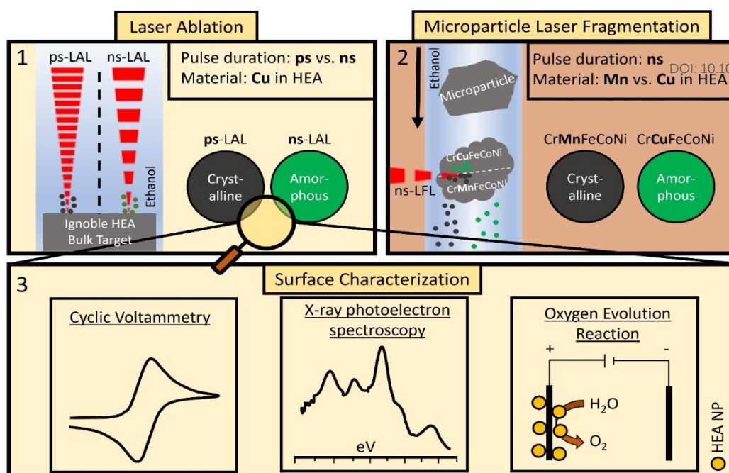
Figure 1. Overview of the study design. (1) Investigation of pulse duration-dependent phase control of CrFeCoNiCu HEA NPs via laser ablation in ethanol, a phenomenon previously addressed for CrMnFeCoNi HEA NPs. 52 (2) Microparticle laser fragmentation in ethanol of CrMnFeCoNi and CrFeCoNiCu microparticles with a high-power ns-pulsed UV laser, studying how the previously observed pulse duration-dependency is transferrable to another, fully-continuous laser-based synthesis technique. (3) Electrochemical surface characterization of crystalline and amorphous CrMnFeCoNi and CrFeCoNiCu HEA NPs (cyclic voltammetry and linear sweep voltammetry) in conjunction with X-ray photoelectron spectroscopy, to study compositional surface changes induced by electrochemical treatment.
