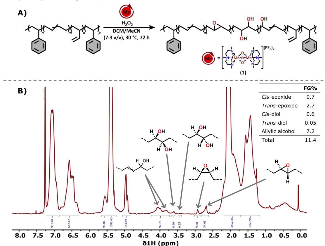
Figure 4: A) Catalytic oxyfunctionalisation conditions tested on SBS using the tri-oxo (1) bridged analogue of MnTACN. B) ^1\text{H} NMR spectrum after the oxyfunctionalisation of styrene-butadiene-styrene (SBS) block-co-polymer, with the corresponding FG% of each installed oxyfunctional group.
