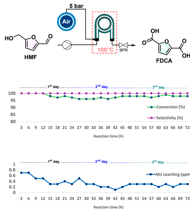
Figure 3. Conversion, selectivity and leaching profile of the 3-day flow session
