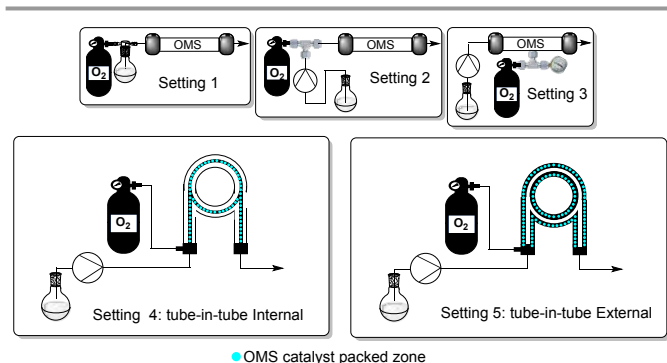
Figure 2. Flow configurations tested.
