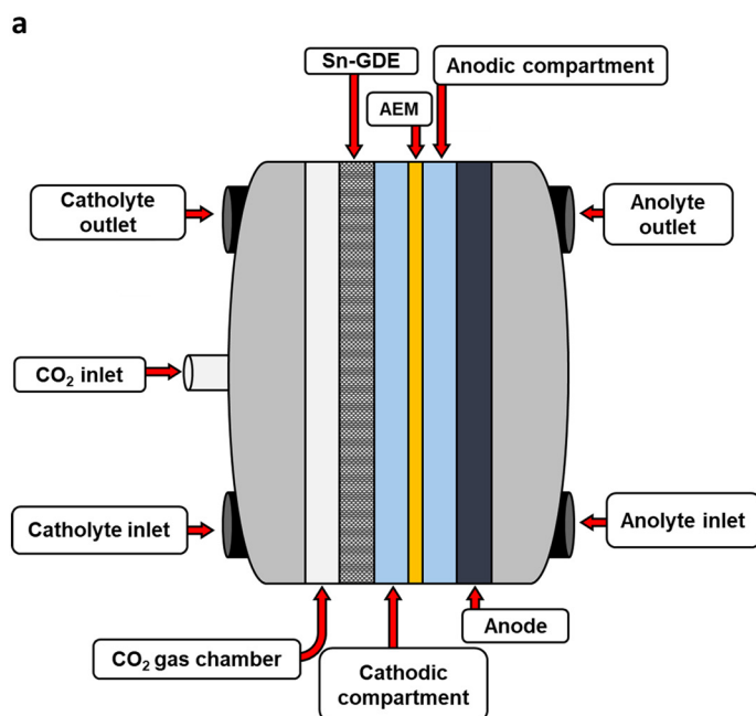
Fig. 10 (a) Schematic and (b) image of the 400 \text{ cm}^2 GDE reactor used in this study.
