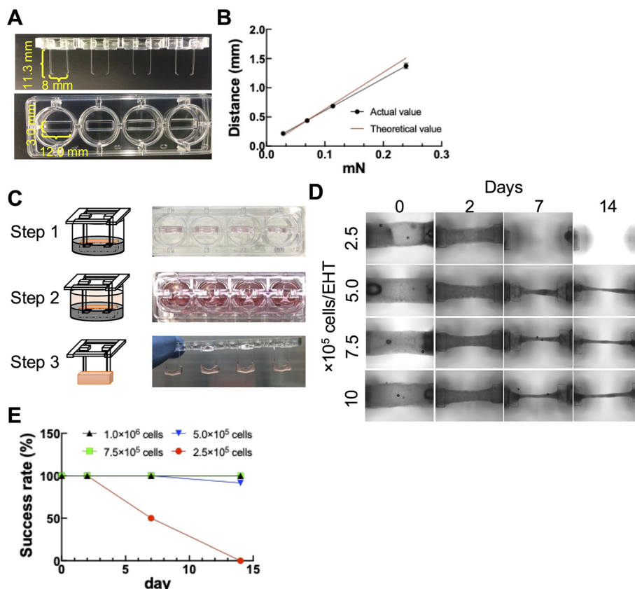
Fig. 2 Generation of PS film-based low-absorption devices. (A) Representative images of a PS film-based device (upper panel) and casting mold container (lower panel). (B) The relationship between pillar displacement and applied force (black line) ( n = 8 ) and theoretical values (red line). (C) Illustration and representative images at each step during EHT construction. Step 1: cell mixtures were seeded into troughs of the casting mold container and incubated for 1 hour. Step 2: IMDM was added after incubation to remove EHTs easily from the casting mold container. Step 3: attached EHTs were removed from the device and transferred into new 24-well plates. (D) Representative images of EHTs at days 0, 2, 7, and 14 after EHT construction. (E) Success rates of EHT generation at days 0, 2, 7, and 14 after EHT construction from 4 independent experiments ( n = 10-12 ).
