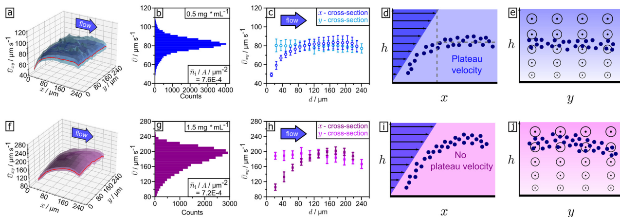
Fig. 6 Spatial mean velocity profile (x–y-plane) for (a) blue (455 nm) and (f) UV (365 nm) illumination for 5 μm sized microparticles. Velocity distributions for (b) blue and (g) UV light. (c) Cross-sections at red lines in 3D profile (a) in x-direction (dark blue) and y-direction (light blue). (h) Cross-sections at red lines in 3D profile (f) in x-direction (dark violet) and y-direction (light violet). All subfigures were either drawn or plotted from tracking results of the measurements shown in Video S4† at steady state (recording time from 10 to 45 s). Cross-sectional visualization of hovering height distribution in x-projection for (d) blue and (i) UV irradiation. Cross-sectional visualization of hovering height distribution in y-projection for (e) blue and (j) UV light. “Circle and point”-signs illustrate the strength of the flow pointing out of plane.
