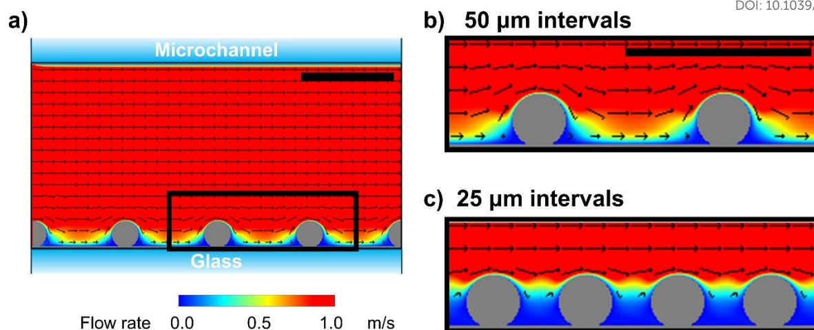
Fig. 3 Physical simulation of the flow rate around arrayed cells. (a) Whole image of the microchannel from the side view with size and flow rate conforming to the real scale. (b–c) Enlarged view of the black square region in (a) under the following conditions: (b) Flow rate = 1.7 m/s and cell interval = 50 \mu\text{m} and (c) flow rate = 1.7 m/s and cell interval = 25 \mu\text{m} . Model cells are set as immovable solid spheres. Flow direction is left to right. Scale bars, 50 \mu\text{m} .
