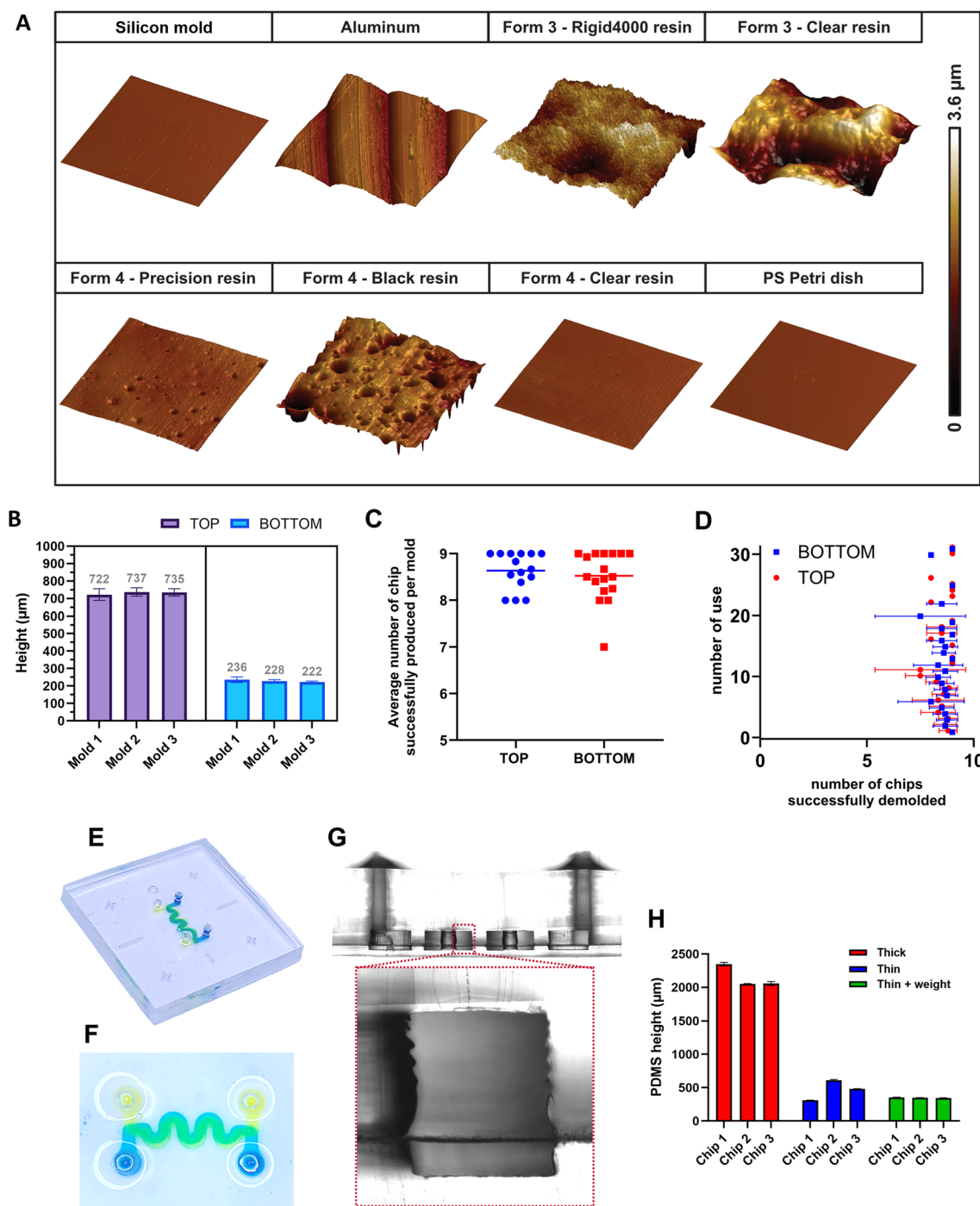
Fig. 2 3D printed mold characterization. A) Topography of PDMS slabs casted on either a silicon mold, PS Petri dish, micromachined aluminum mold or 3D printed molds. Scan size: 100\ \mu\text{m}^2 B) channel height measurements within the same mold of between different batches. C) Graph of the average number of chips produced per molds, one point is one iteration. D) Evaluation of the performance of the molds across time. E) and F) Views of the final 3D \mu -Gut device, top channel in yellow and bottom channel in blue. G) Cross section of the resulting PDMS chip. H) Thickness measurement of the PDMS layer under the BOTTOM channel depending on molding techniques.
