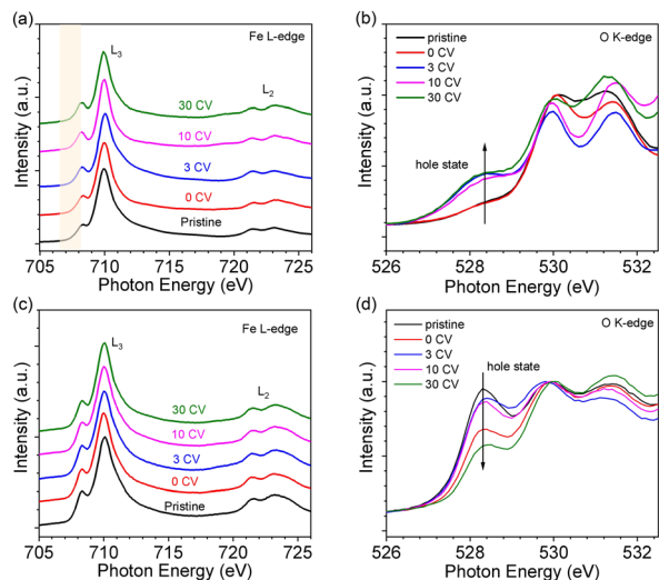
Fig. 2 NEXAFS spectra of \text{LaFeO}_3 and \text{La}_{0.67}\text{Sr}_{0.33}\text{FeO}_3 with different CV cycles. (a) Fe L-edge of \text{LaFeO}_3 , (b) O K-edge of \text{LaFeO}_3 , (c) Fe L-edge of \text{La}_{0.67}\text{Sr}_{0.33}\text{FeO}_3 and (d) O K-edge of \text{La}_{0.67}\text{Sr}_{0.33}\text{FeO}_3 . The yellow bars in (a) indicate the changes in the characteristics of \text{Fe}^{3+} and \text{Fe}^{4+} at 708 eV under different CV cycles.
