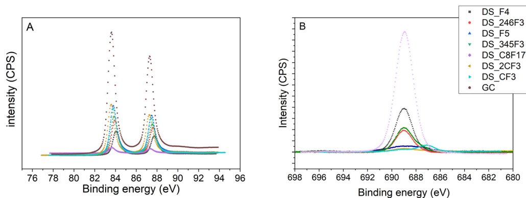
Fig. 8 (A) \text{Au}_{4f} and (B) \text{F}_{1s} core level spectra of Au thin film before and after modification by electrochemical reduction with various aryldiazonium salts.
