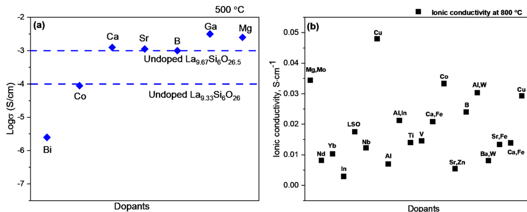
Fig. 10 (a) Comparison of conductivities of different dopants at a constant level of oxygen excess at 500\text{ }^{\circ}\text{C} ; (b) ionic conductivity of different dopants at 800\text{ }^{\circ}\text{C} .
