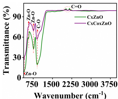
Fig. 7 FTIR spectra of CxZnO and CxCoxZnO thin films.
