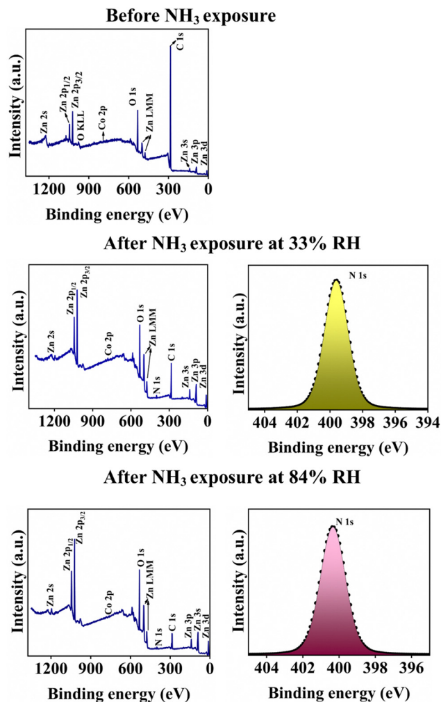
Fig. 18 Survey spectrum and N1s narrow scan spectrum of the CxCoxZnO thin film before and after exposure to ammonia.
