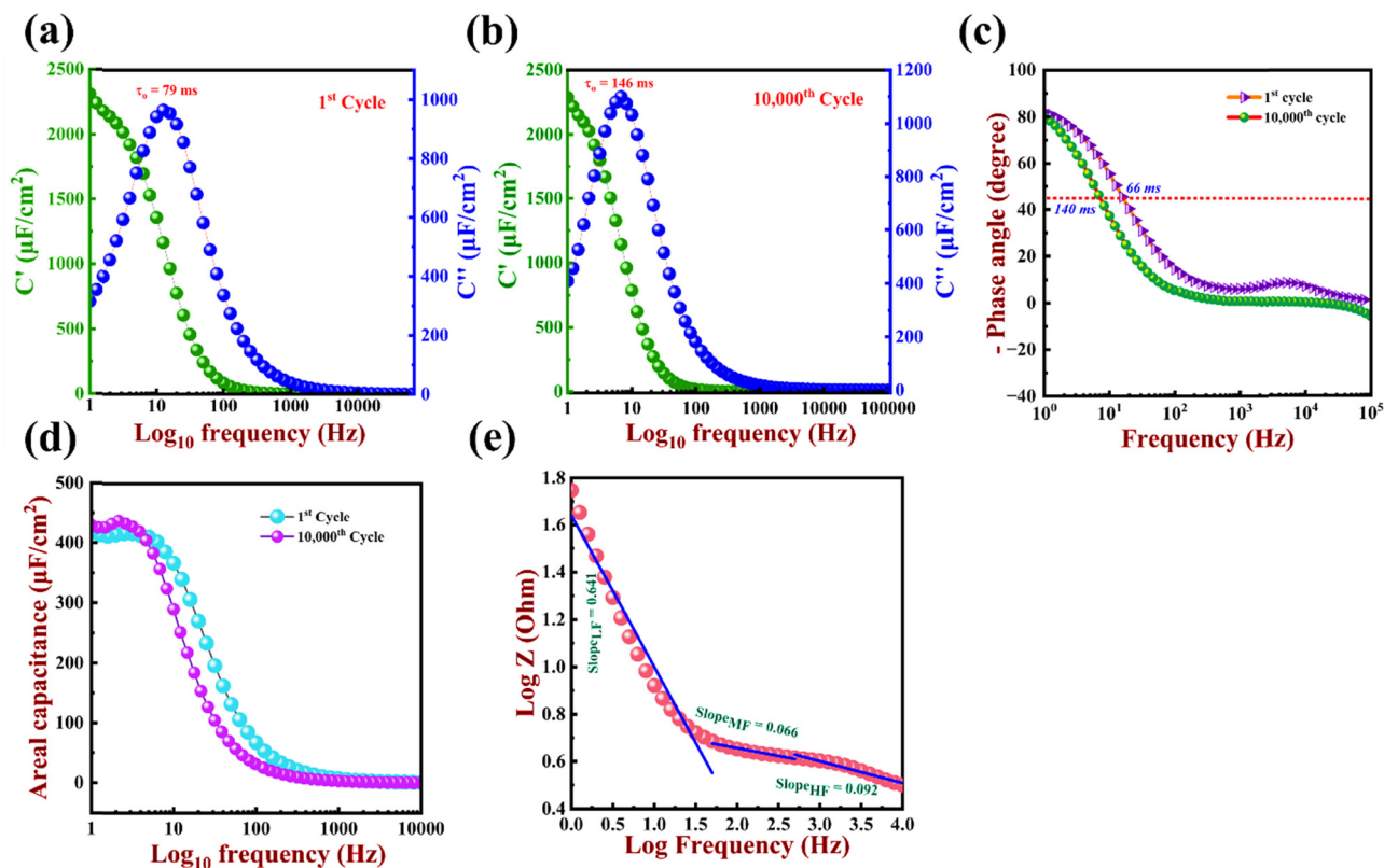
Fig. 11 (a) C' and C'' vs. frequency of CoWO 4 /AC at the 1st cycle. (b) C' and C'' vs. frequency of CoWO 4 /AC at the 10 000th cycle. (c) The phase angle bode plot. (d) Areal capacitance vs. log frequency at the 1st and 10 000th cycle. (e) Impedance bode plot.
