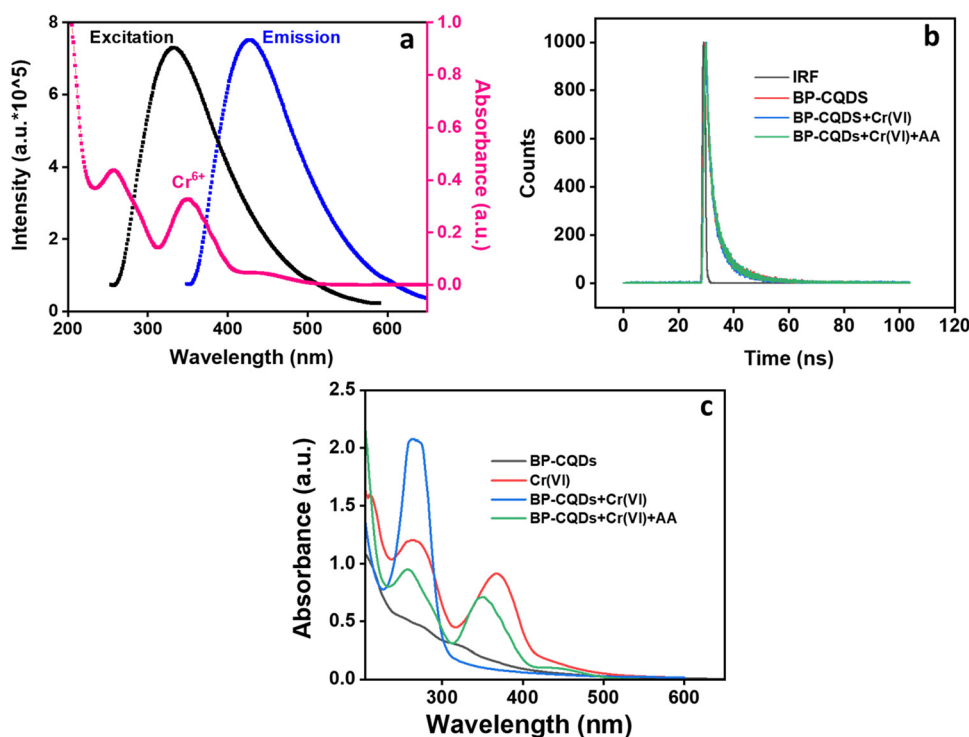
Fig. 4 (a) The absorption spectra of \text{Cr}(\text{vi}) ions overlap with the excitation spectrum of BP-CQDs confirming IFE, (b) fluorescence lifetime decay of BP-CQDs with \text{Cr}(\text{vi}) and AA, and (c) UV-Vis absorption spectrum of BP-CQDs, \text{Cr}(\text{vi}) , BP-CQDs + \text{Cr}(\text{vi}) , and BP-CQDs + \text{Cr}(\text{vi}) + AA.
