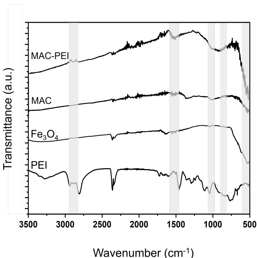
Fig. 4. FTIR analysis of the particles investigated.
