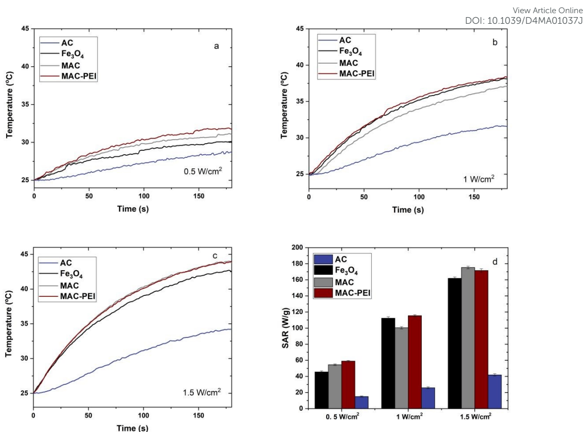
Fig. 6. Temperature increases for PTT therapy, at a power irradiation of 0.5 W/cm 2 (a), 1 W/cm 2 (b), and 1.5 W/cm 2 (c), using 100 \mu L of sample at 5 mg/mL. Determination of the SAR obtained (d).
