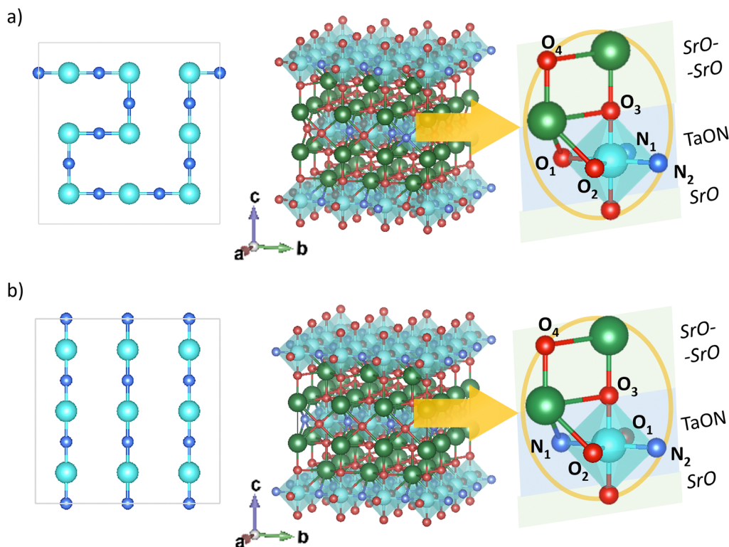
Fig. 4 (a) Representation of anion ordering constructable with the most cis -character; 6/9 \text{N}^{3-}-\text{Ta}^{5+}-\text{N}^{3-} chains are cis - and 3/9 are trans - and (b) corresponding fully trans -ordering used for the 3 \times 3 \times 1 supercell. Insets depict anion/vacancy positions from the core of the structure used in this work, which also map to the 2 \times 2 \times 1 supercell.
