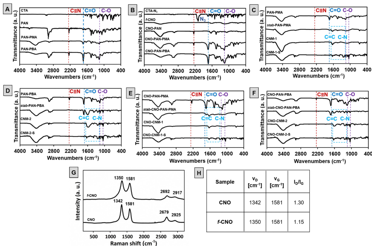
Fig. 3 (A)–(F) The FTIR spectra of a chain transfer agent, PAN-polymer, PAN-polyacrylate copolymers, and their composites before and after thermal treatment; (G) Raman spectra of CNO and f-CNO; and (H) the frequencies for the G and D bands and their relative intensities ( I_D/I_G ) for CNO and f-CNO excited at 514 nm.
