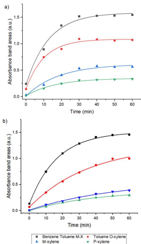
Fig. 5 Dependence of the IR absorbance band area on time using 5 \mu\text{m} (a) P3HB4HB and (b) PHO polymer films to analyse 50 ppm BTX solution at a flow rate of 3 mL min -1 .
