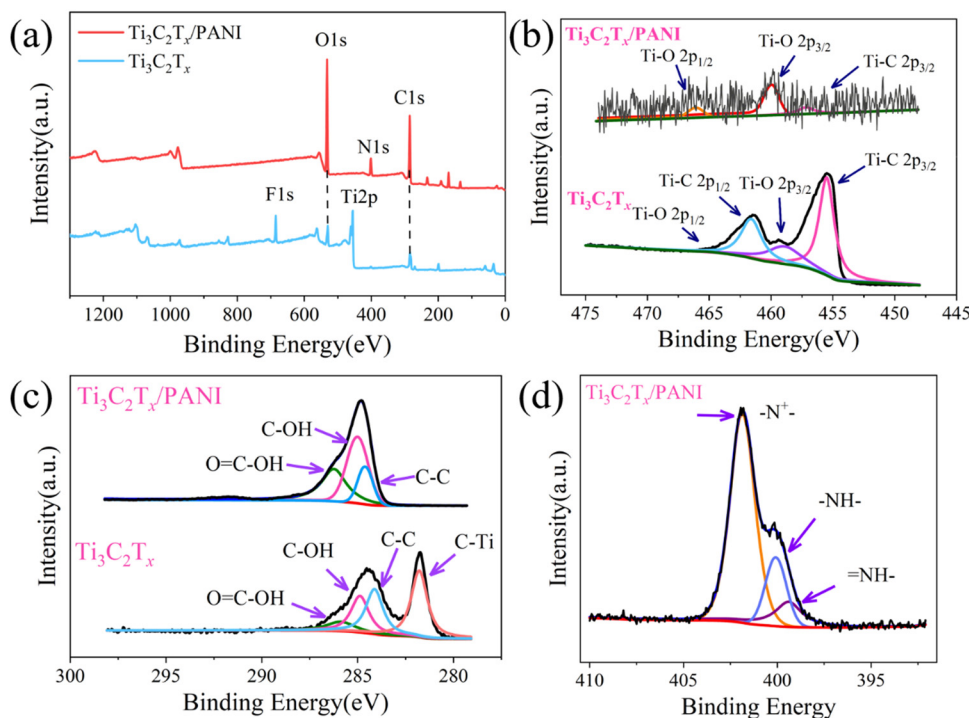
Fig. 4 The XPS spectra of Ti_3C_2T_x and Ti_3C_2T_x/PANI . (a) The survey spectra of Ti_3C_2T_x and Ti_3C_2T_x/PANI and the high resolution XPS spectra of (b) Ti 2p, (c) C 1s and (d) N 1s for Ti_3C_2T_x and Ti_3C_2T_x/PANI .
