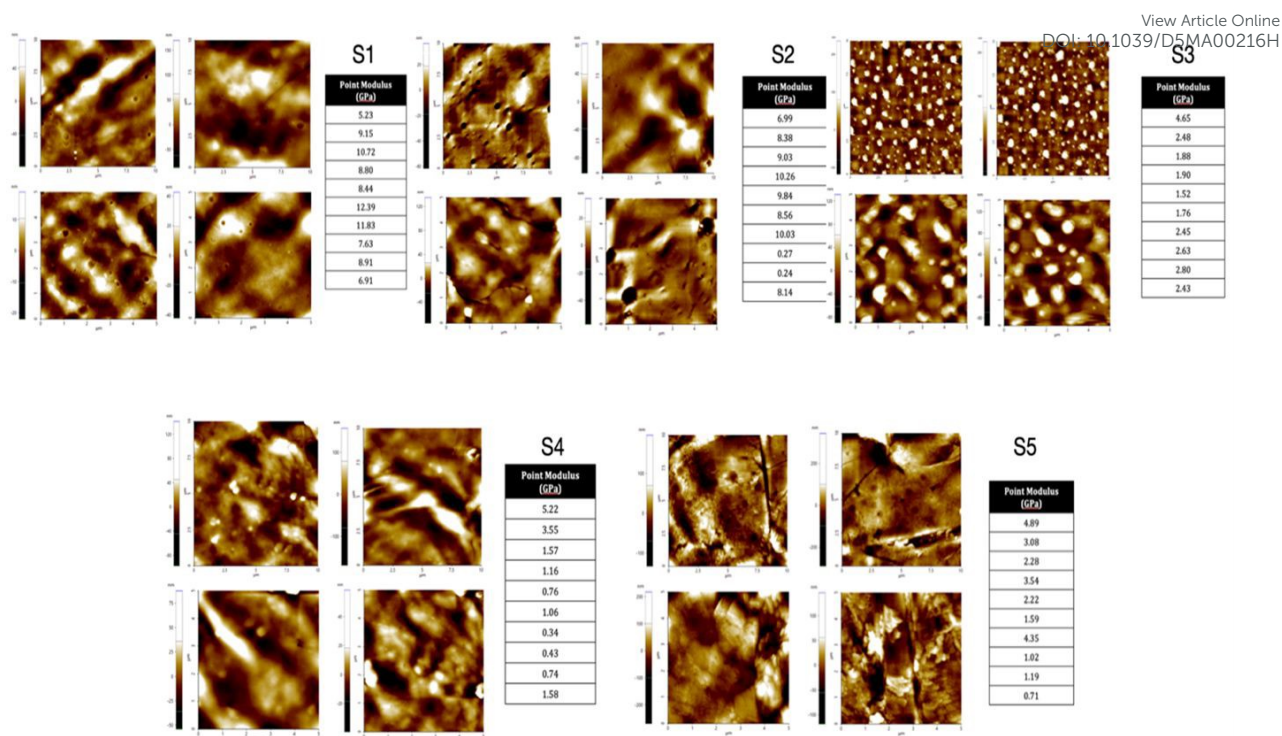
Figure 1. Atomic Force Microscopic analysis of different polyesters (S1-S5)
