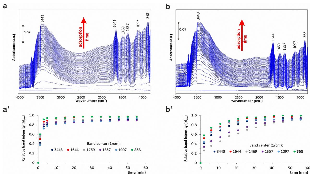
Fig. 6 Spectral changes induced by H_2O adsorption on (a) nW-CuO(200) and (b) nW-CuO(25). The bottom panels (a') and (b') collect the quantitative data (note that p/p_s = 0.9 , in Ar with a total flow rate of 50\text{ mL min}^{-1} was used).
