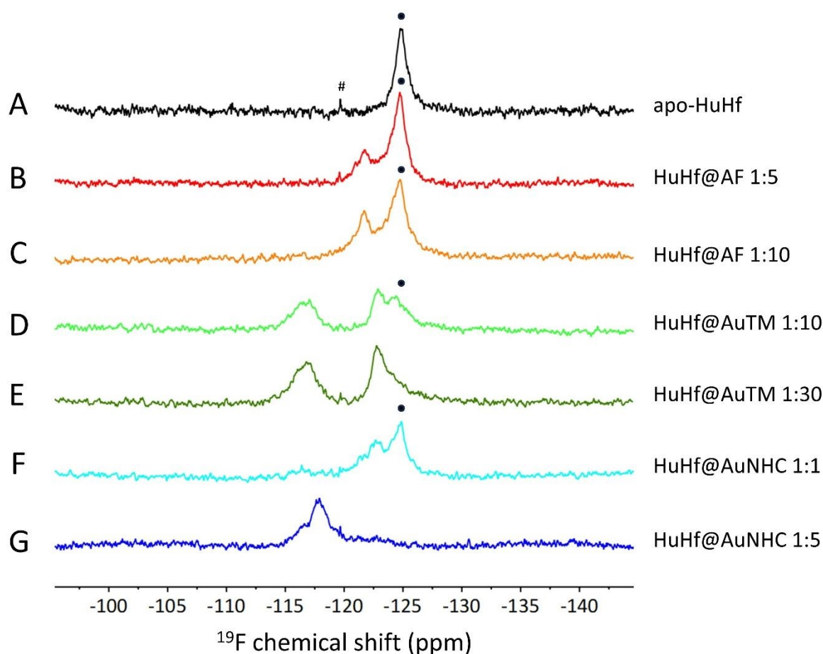
Figure 2. ^{19}\text{F} NMR spectra of HuHf gold(I)-bioconjugates (15 \mu\text{M} ) recorded at 14.1 T and 298 K; A) apo-HuHf; B-C) HuHf@AF; D-E) HuHf@AuTM; F-G) HuHf@AuNHC. ^{19}\text{F} chemical shifts were referenced to trifluoroacetic acid, used as an external standard (0 ppm). The ratios are given as subunit:compound, so, for example, a 1:10 ratio indicates that 10 equivalents of compound were added per ferritin subunit (i.e. per binding site), corresponding to 240 equivalents per cage. The black dot indicates the NMR signal of the apo form of the protein; #: contaminant.
