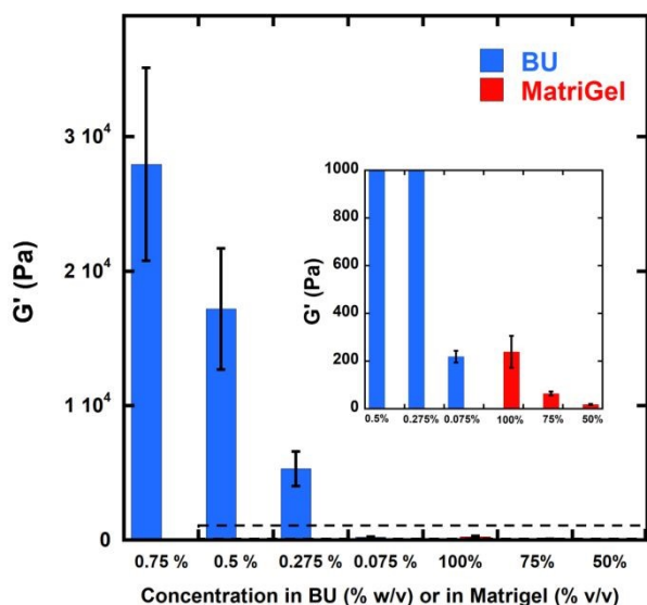
Figure 2: Elastic moduli ( G' ) values recorded at a sweep frequency of 1Hz. G' of GNBA (BU) based supramolecular gels (Blue) versus Matrigel (red) are reported at different concentrations (BU % w/v, Matrigel %v/v).
