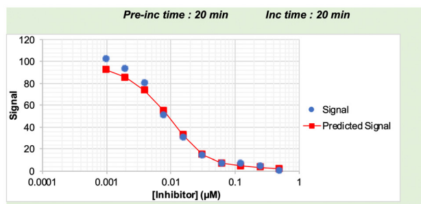
Fig. 8 Global fitting of pre-incubation time dependent IC_{50} datasets obtained for saxagliptin, using EPIC-CoRe. IC_{50} curves were obtained for pre-incubation times ranging from 0–20 min and incubation times fixed at 20 min.
