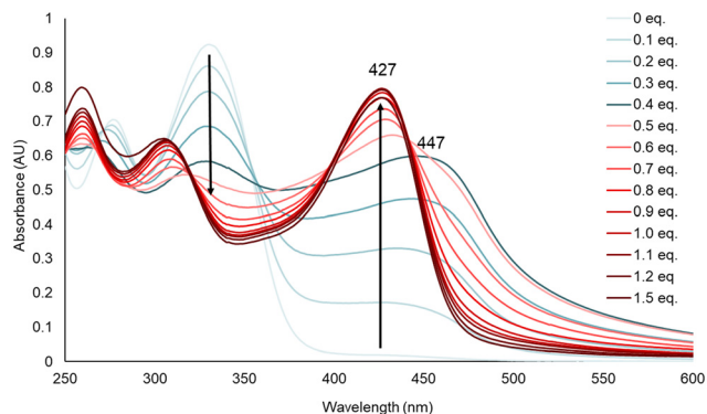
Fig. 4 UV/vis absorption profile acquired by titrating \text{CuSO}_4 to 50 \mu\text{M} in 75 \text{ mM} Tris-HCl buffer at pH 7.4. Absorption maximum shifts from 447 \text{ nm} at 0.4 \text{ equiv.} to 427 \text{ nm} at 1.0 \text{ equiv.}
