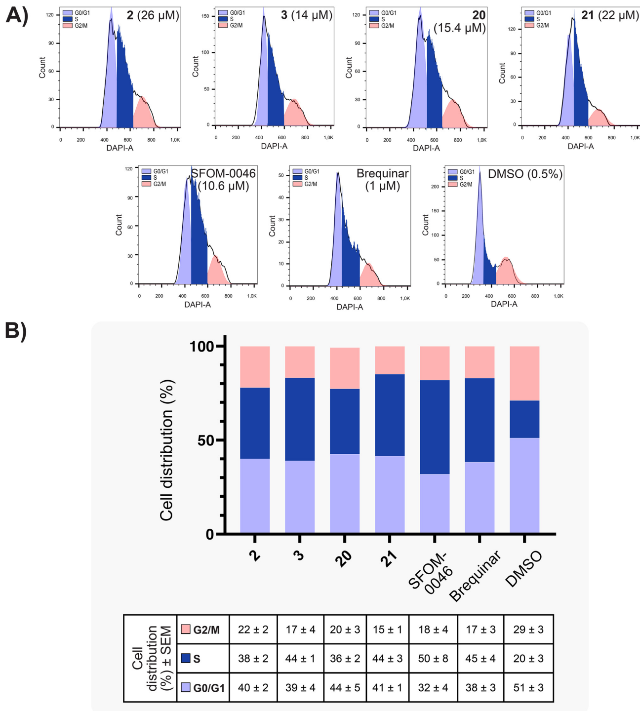
Fig. 2 A) Effects of PYRUB-SOs 2 and 3 and their corresponding hydrochlorides 20 and 21 on the cell cycle progression of non-AML M21 cells. SFOM-0046 and brequinar were used as positive controls, while 0.5% DMSO was used as the excipient. B) Histogram displaying cell cycle distribution.
