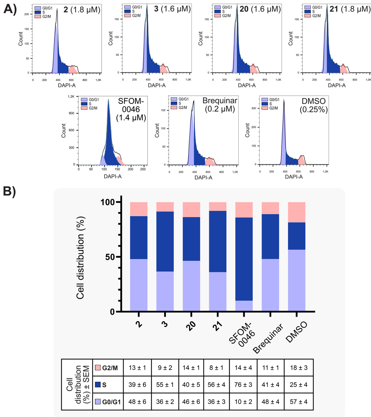
Fig. 3 A) Effects of PYRUB-SOs 2 and 3 and their corresponding hydrochlorides 20 and 21 on the cell cycle progression of AML MOLM-13 cells. SFOM-0046 and brequinar were used as a positive control, while 0.25% DMSO was used as the excipient. B) Histogram displaying cell cycle distribution.
