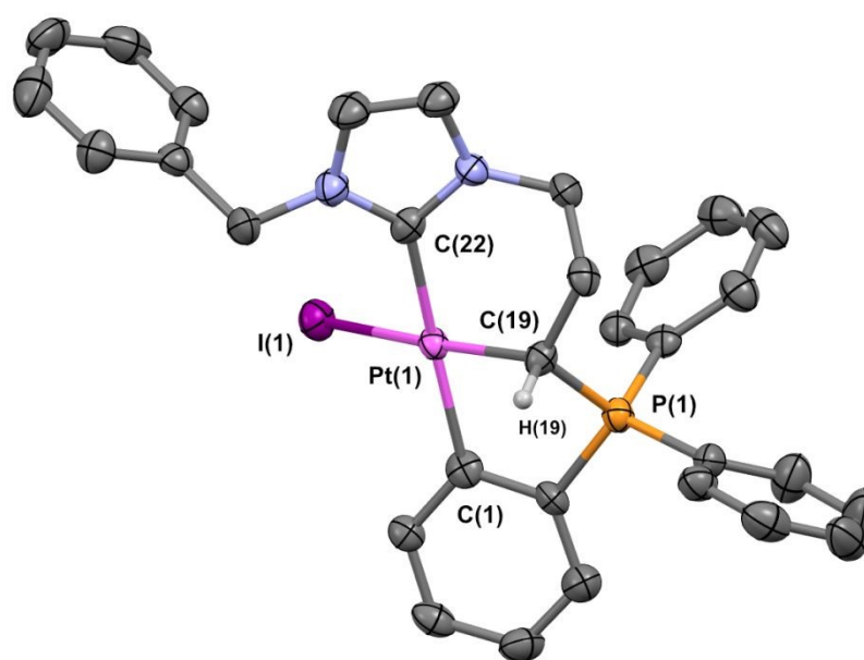
Figure 3. ORTEP view of ortho-metalated complex 5 . Thermal ellipsoids set at the 60% probability level, hydrogen atoms are omitted, except of the ylide function. Selected distances (Å) and angles (°): C(22)-Pt(1), 2.049(3); C(1)-Pt(1), 2.067(3); Pt(1)-I(1), 2.688(3); C(19)-Pt(1), 2.091(3); P(1)-C(19), 1.788(3); C(22)-Pt(1)-I(1), 94.82(9), C(22)-Pt(1)-C(19), 88.17(13); C(1)-Pt(1)-I(1), 92.24(9); C(1)-Pt(1)-C(19), 85.49(13); C(22)-Pt(1)-C(1), 171.95(13); I(1)-Pt(1)-C(19), 170.22(9). CCDC-2373163.
