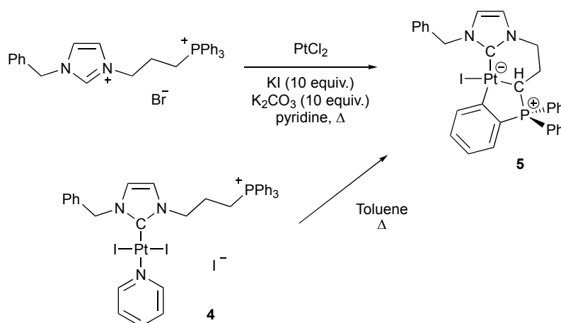
Figure 2. Observed double C-H activation upon heating the triphenylphosphonium-functionalized Pt NHC complex 4 or direct synthesis of 5 starting from the corresponding imidazolium precursor.
