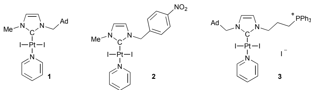
Figure 1. Molecular structure of the synthesized NHC platinum complexes 1-3 . Complexes 1 and 2 were obtained in a one-step procedure from the corresponding imidazolium, PtCl 2 , KI, K 2 CO 3 in pyridine (100 °C). Complex 3 was obtained in two steps starting from the imidazolium, PtCl 2 (SMe 2 ), KI, K 2 CO 3 in acetone (R.T.), followed by pyridine/SMe 2 ligand exchange at room temperature.
