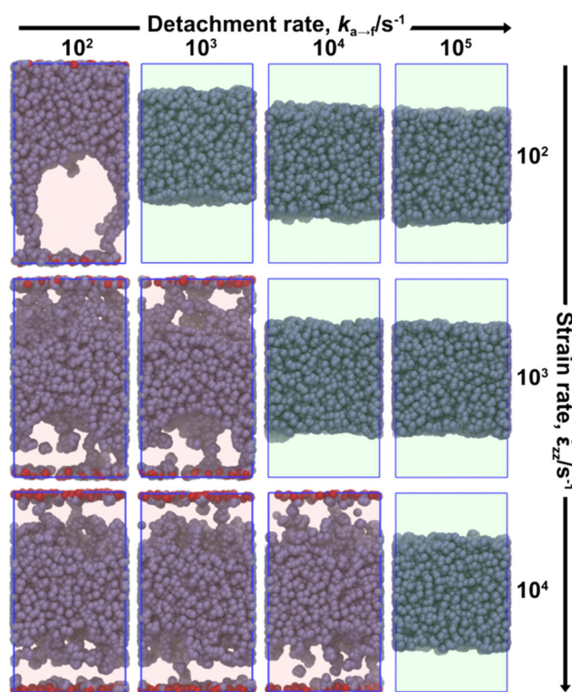
Fig. 9 Snapshots of the final mesoscopic configurations at various detachment rates (increasing from left to right) and elongation rates (increasing from top to bottom) for K_{\text{ads}} = 1/4 . Green/red shaded plots indicate total/partial detachment until \epsilon_{\text{max}} = 1 .
