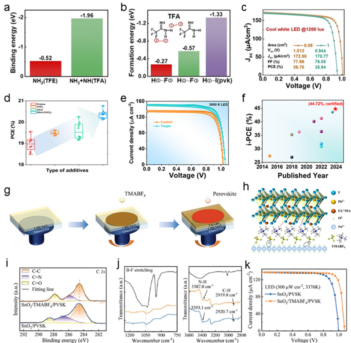
Fig. 4 (a) The comparative calculated binding energies of \text{NH}_2\text{-Pb}^{2+} and \text{NH}_4^+\text{NH}_2\text{-Pb}^{2+} for TFE and TFA, respectively. And (b) the calculated formation energies of \text{H-O-F} , \text{H-O-F} , and \text{H-O-I} (perovskite) interactions for TFA. And (c) J - V curves of TFA- \text{CsPbI}_{3-x}\text{Br}_x -based solar cells with effective cell areas of 0.09 and 1.0 \text{cm}^2 under 1200 lux ( 341 \mu\text{W cm}^{-2} ) illumination. Reproduced with permission. 60 Copyright 2022, John Wiley and Sons. (d) Statistical deviations of PCE for WBG PSCs incorporating various additives. And (e) J - V curves representing IPVs performance of control and target WBG PSCs under LED light at 1000 lux. And (f) summary of i-PCEs from representative studies (2014–2023). Reproduced with permission. 57 Copyright 2024, Royal Society of Chemistry. (g) Deposition procedure for the solar cells. (h) Schematic diagram of the bridge function at the buried interface. (i) C 1s XPS spectra of the control and target films. (j) FTIR spectra of \text{TMABF}_4 (black), perovskite based on \text{SnO}_2 (yellow) and \text{SnO}_2/\text{TMABF}_4 (blue). (k) Champion device J - V curves of the control and target devices under 300 \mu\text{W cm}^{-2} LED light. Reproduced with permission. 103 Copyright 2024, John Wiley and Sons.
