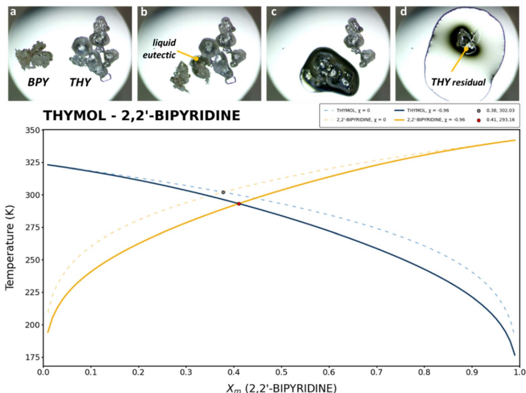
Fig. 3 Top: optical microscopy images at 100× magnification for thymol (THY) : 2,2' bipyridine (BPY) binary mixture collected under ambient conditions. (a) Separated crystals of the chemical species. (b) A liquid eutectic phase is observed when they are put in contact. (c) The liquid eutectic phase grew until the minor component is still present. (d) Residual solid thymol embedded within the eutectic liquid phase. Bottom: PoEM output from the single-plot plugin: Schroeder-van Laar's curve plotted for THY for \chi = 0 (dashed blue line) and \chi = -0.96 (solid blue line) and for BPY for \chi = 0 (dashed orange line) and \chi = -0.96 (solid orange line). Eutectic point calculated under the ideal conditions (grey point, \chi = 0 ) and under real conditions (red point, \chi = -0.96 ).
